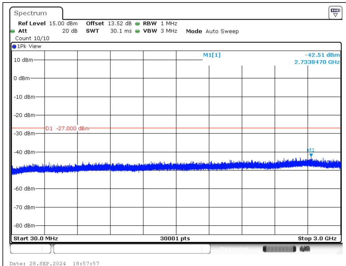
11AX160MIMO-Ant2-6025-30~3000-PASS
