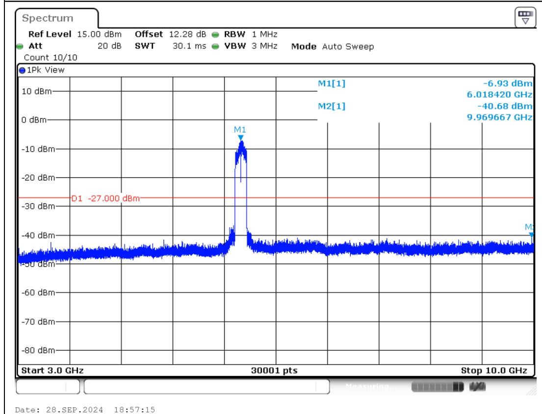
11AX160MIMO-Ant1-6025-3000~10000-PASS
