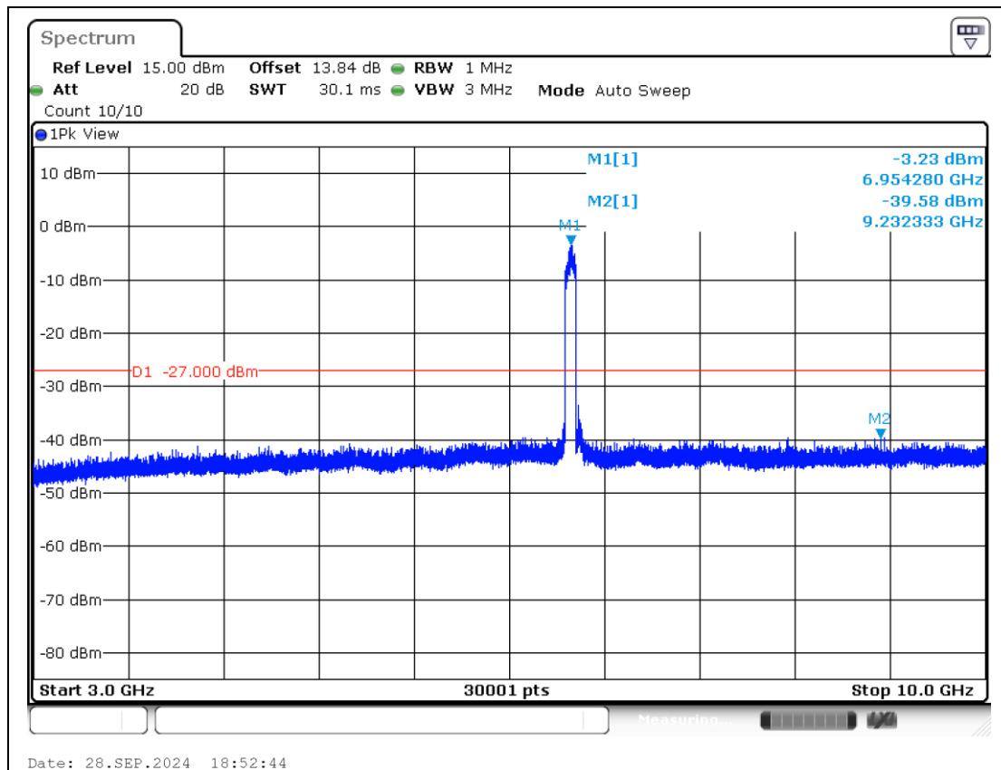
11AX80MIMO-Ant2-6945-3000~10000-PASS
