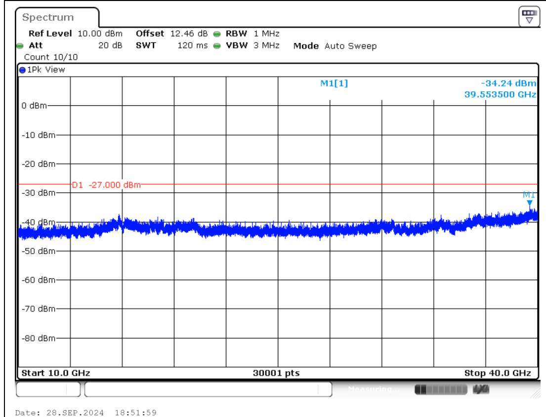
11AX80MIMO-Ant1-6945-10000~40000-PASS
