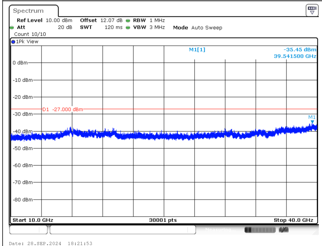
11AX80MIMO-Ant1-5985-10000~40000-PASS
