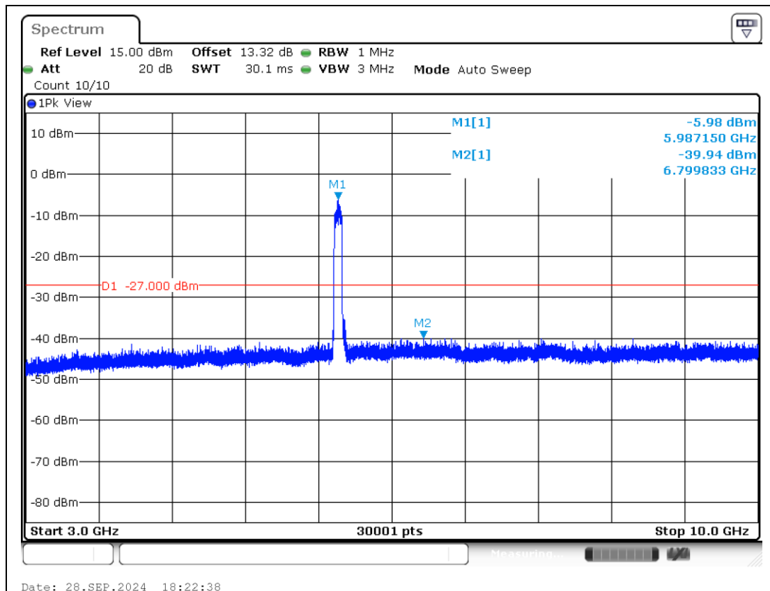
11AX80MIMO-Ant2-5985-3000~10000-PASS
