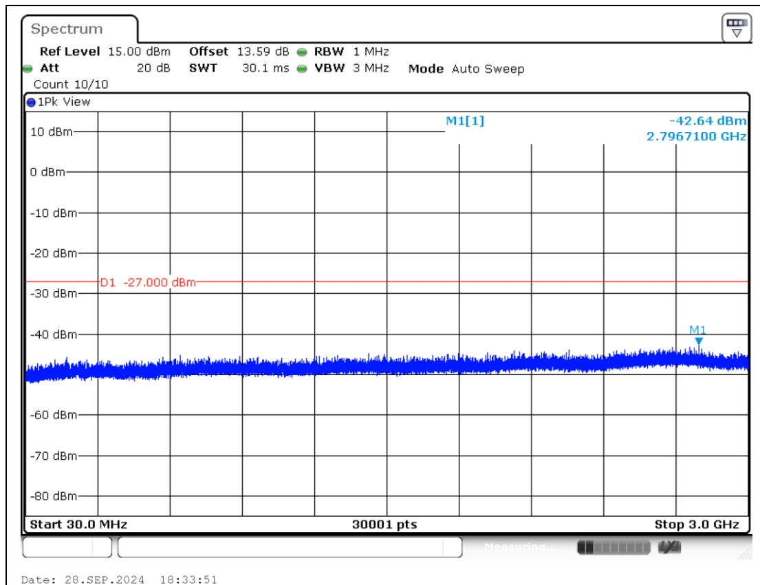
11AX80MIMO-Ant2-6545-30~3000-PASS
