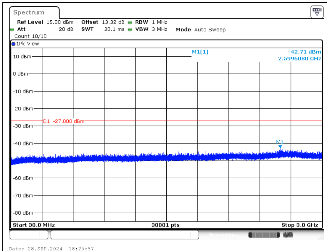
11AX80MIMO-Ant2-6145-30~3000-PASS
