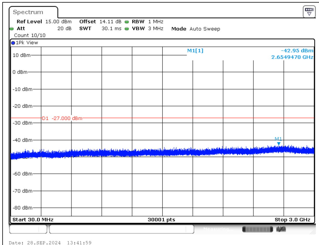
11AX20MIMO-Ant2-6855-30~3000-PASS
