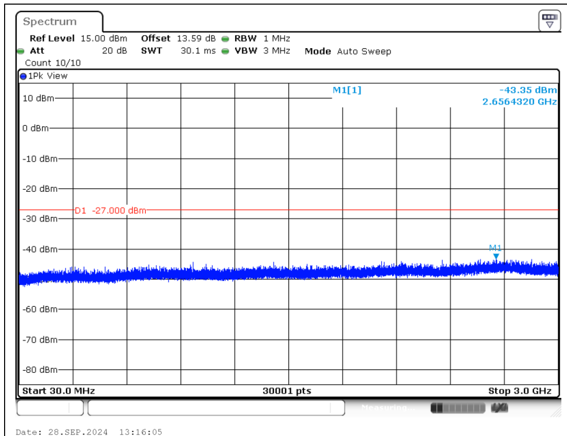
11AX20MIMO-Ant2-6515-30~3000-PASS
