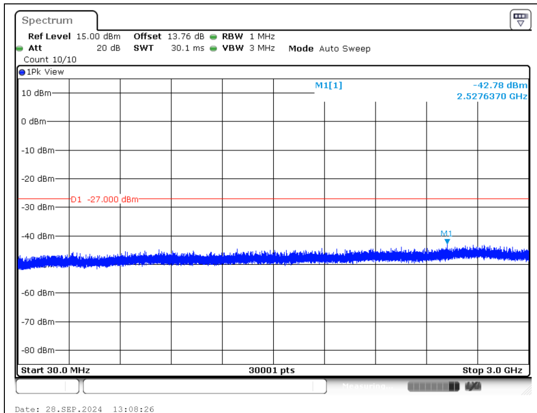
11AX20MIMO-Ant2-6435-30~3000-PASS
