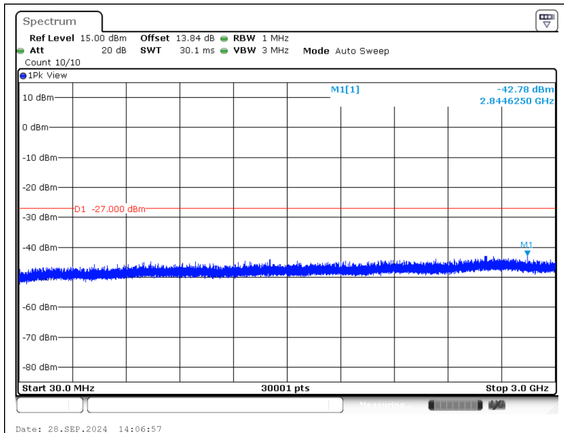
11AX20MIMO-Ant2-6995-30~3000-PASS
