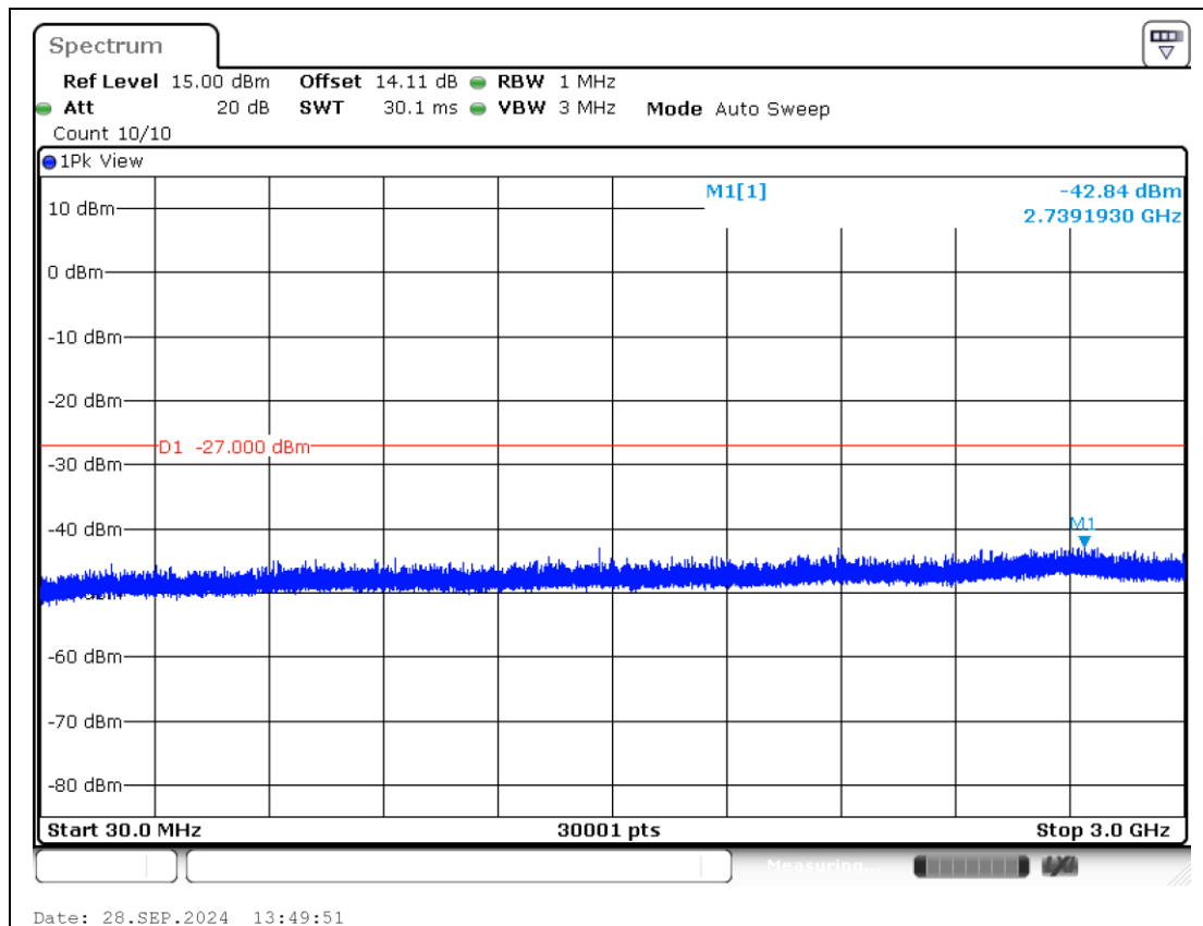
11AX20MIMO-Ant2-6875-30~3000-PASS
