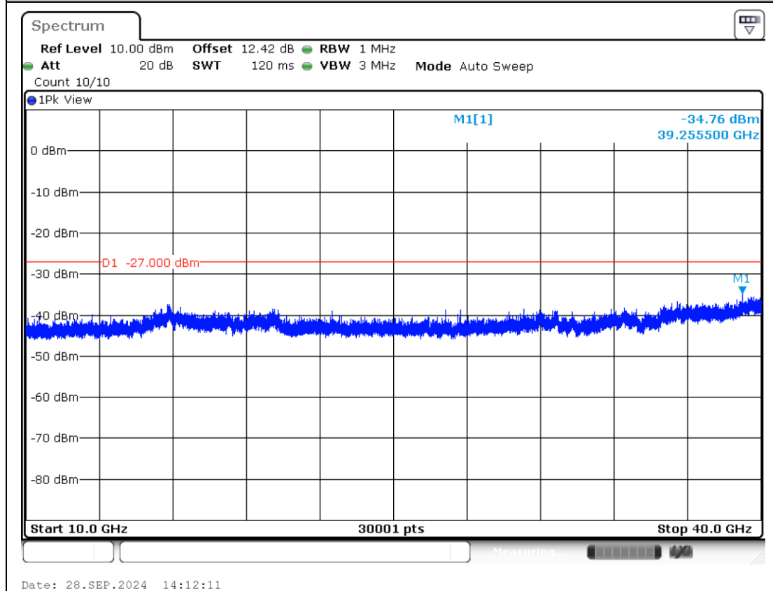
11AX20MIMO-Ant1-7115-10000~40000-PASS
