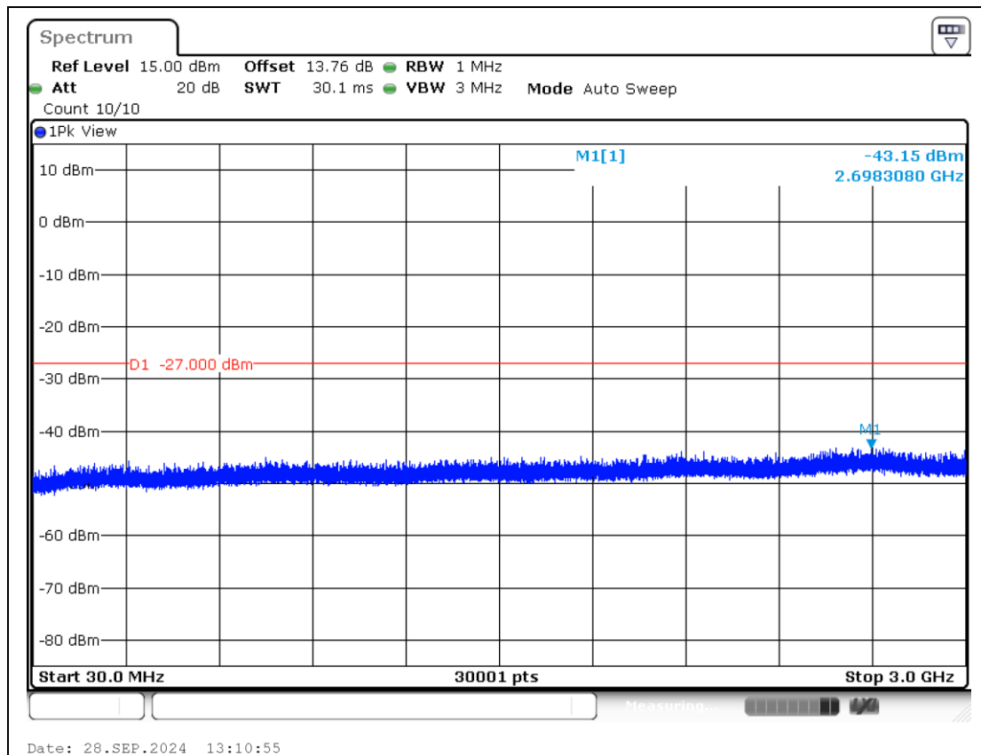
11AX20MIMO-Ant2-6475-30~3000-PASS
