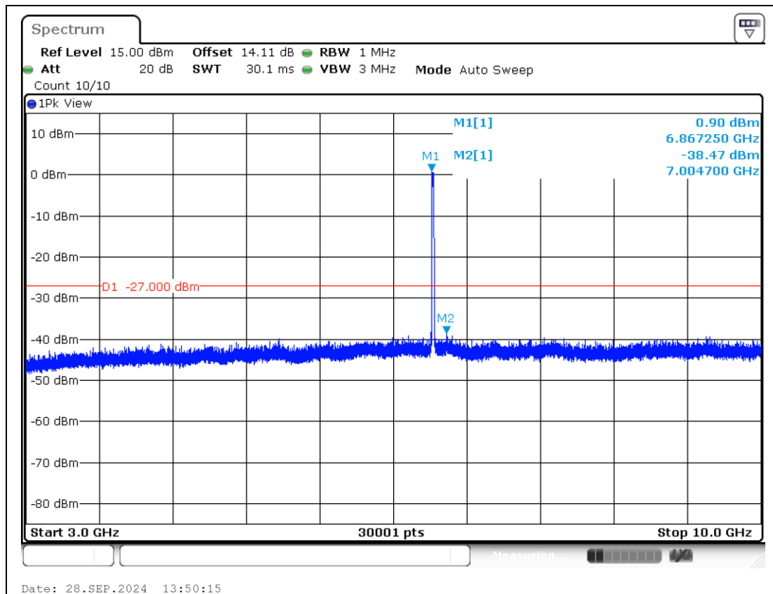
11AX20MIMO-Ant2-6875-3000~10000-PASS
