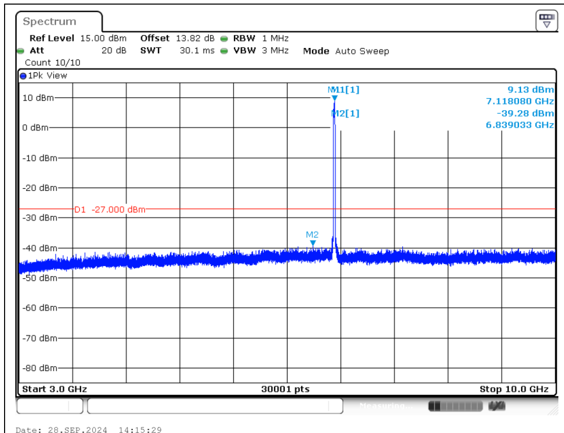
11AX20MIMO-Ant2-7115-3000~10000-PASS
