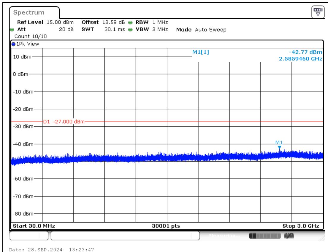
11AX20MIMO-Ant2-6535-30~3000-PASS
