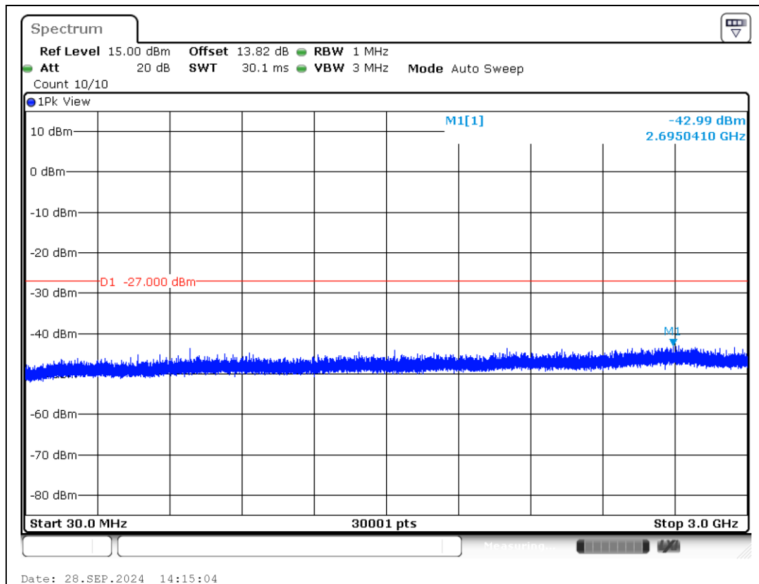
11AX20MIMO-Ant2-7115-30~3000-PASS
