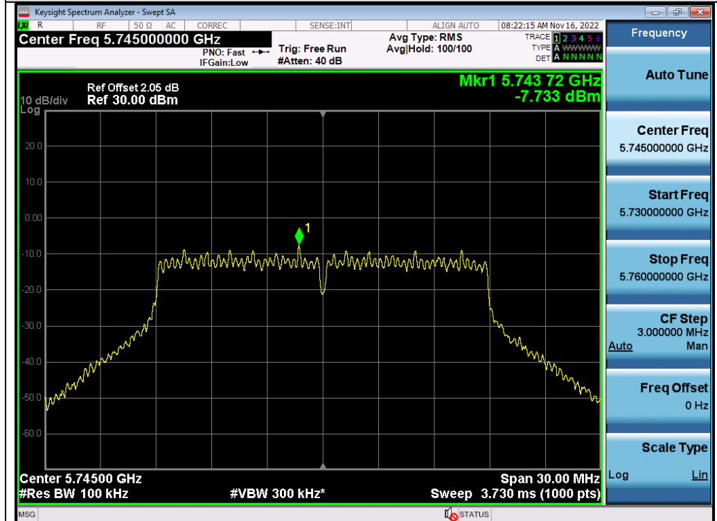
Test_Graph_802.11n20_ANT2_5745_MCS0_PSD
