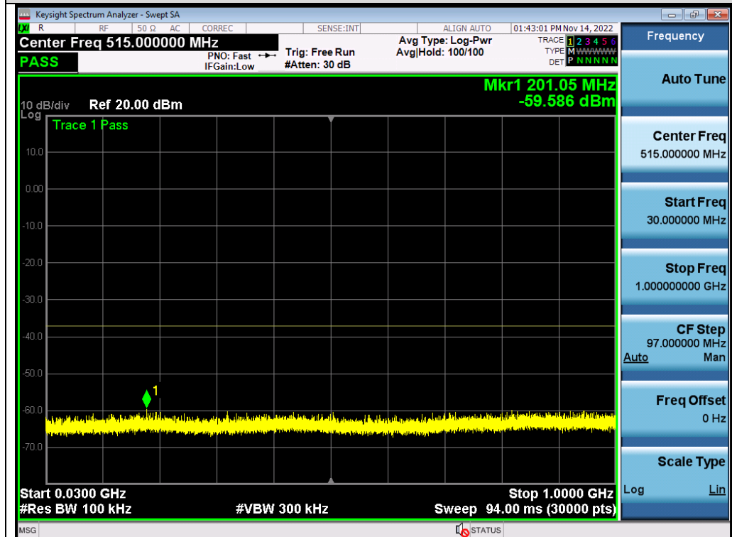
Test_Graph_802.11n40_ANT1_5230_MCS0_Frequency Band 1
