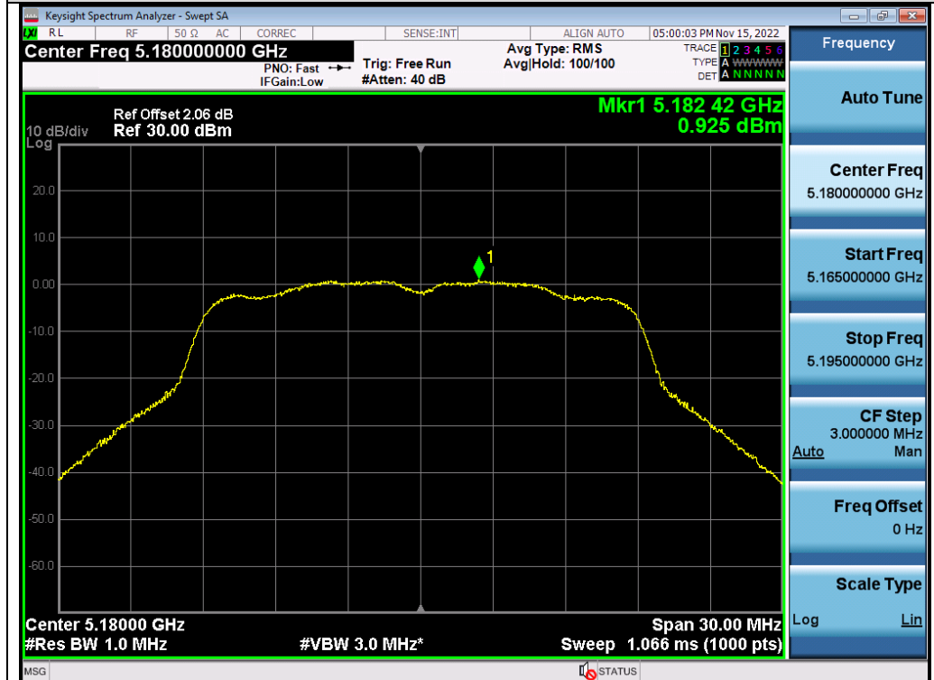
Test_Graph_802.11n20_ANT2_5180_MCS0_PSD
