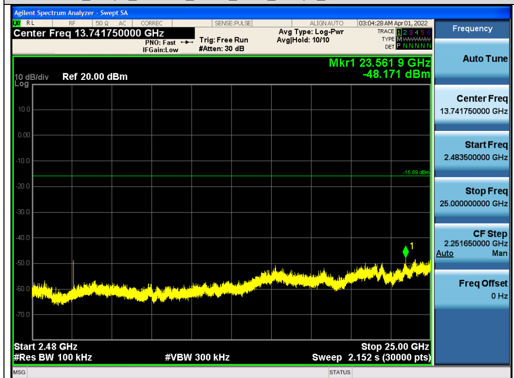
Test Graph 802.11b ANT2 2412 1Mbps Higher Band Emissions
