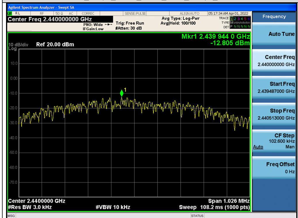
Test_Graph_LE1M_ANT2_2440_1Mbps_PSD
