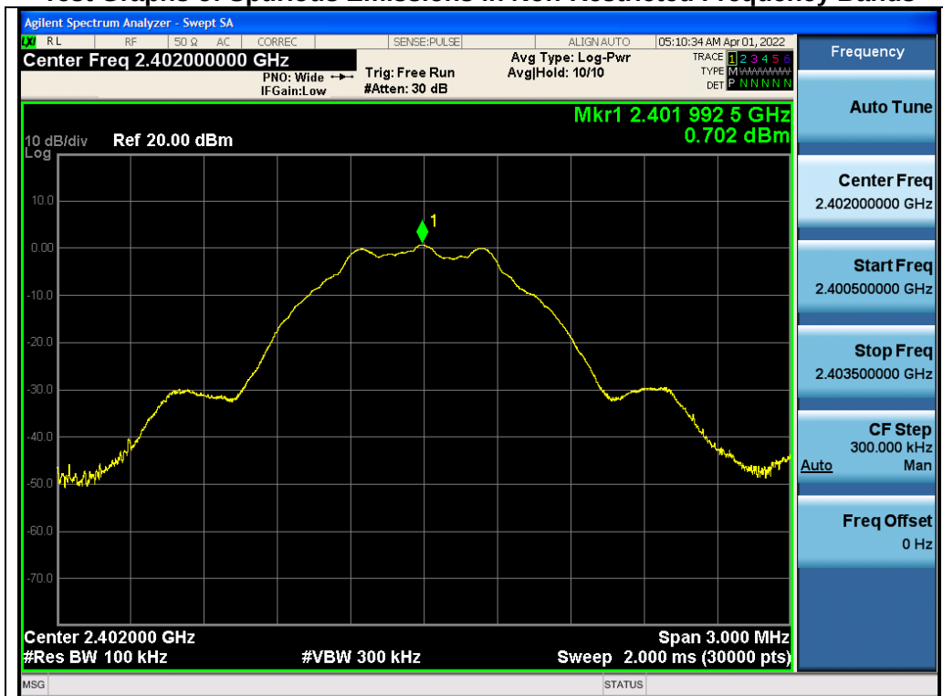
Test_Graph_LE1M_ANT2_2402_1Mbps_Reference Level
