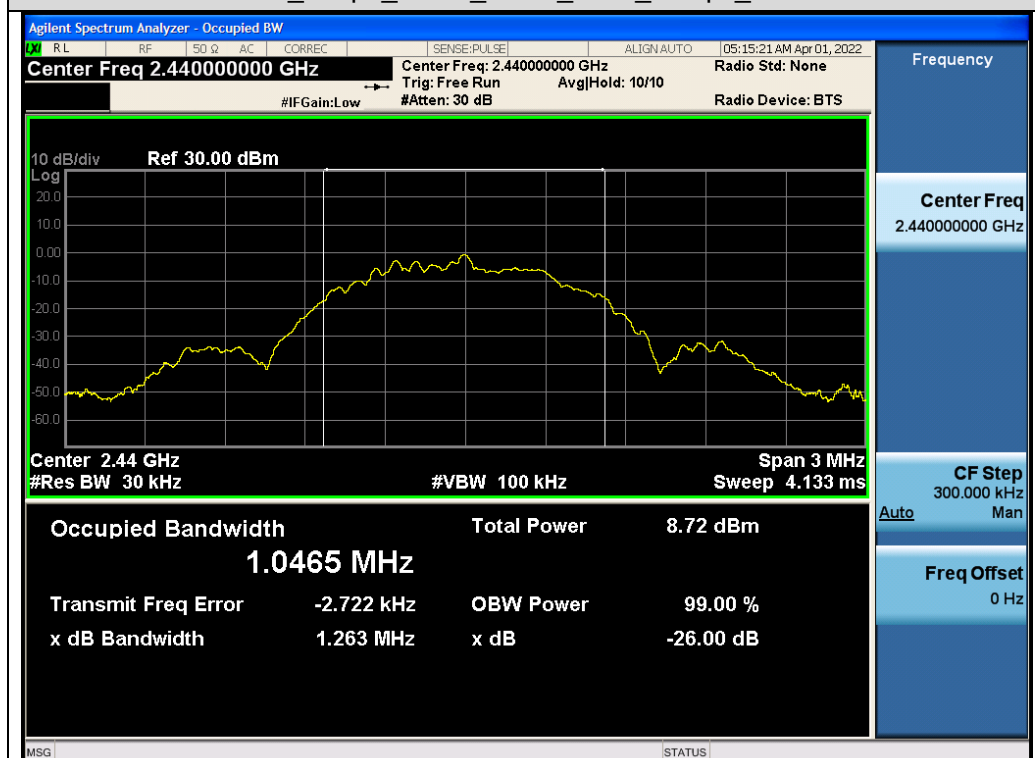
Test_Graph_LE1M_ANT2_2440_1Mbps_OBW
