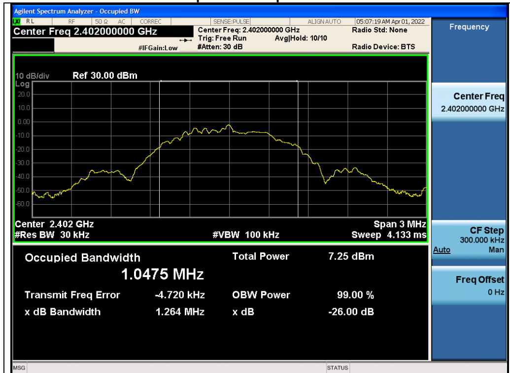
Test_Graph_LE1M_ANT2_2402_1Mbps_OBW
