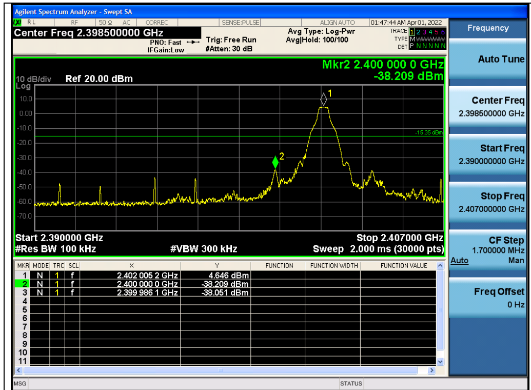
Test_Graph_BR_ANT2_2402_1Mbps_Lower Band Edge Emissions
