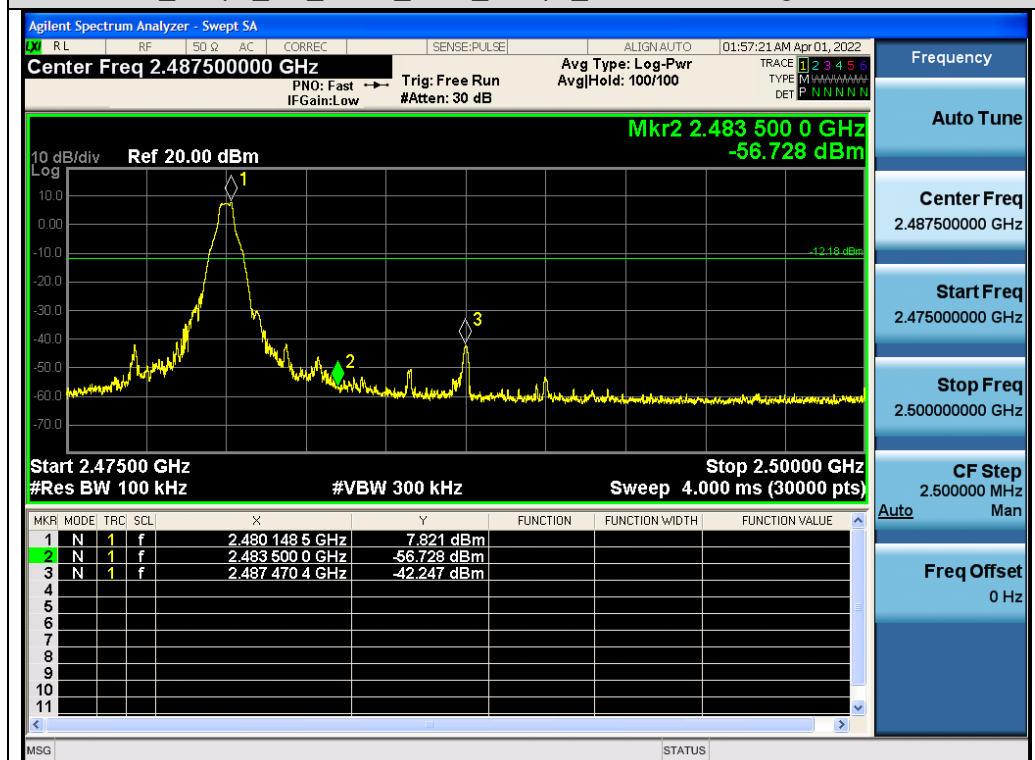
Test_Graph_BR_ANT2_2480_1Mbps_Higher Band Edge Emissions
