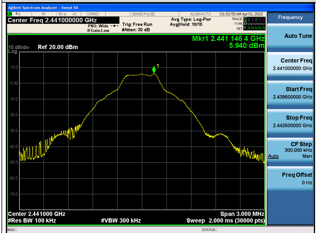
Test_Graph_BR_ANT2_2441_1Mbps_Reference Level
