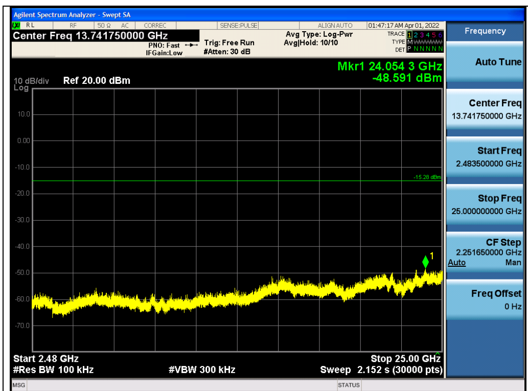
Test_Graph_BR_ANT2_2402_1Mbps_Higher Band Emissions
