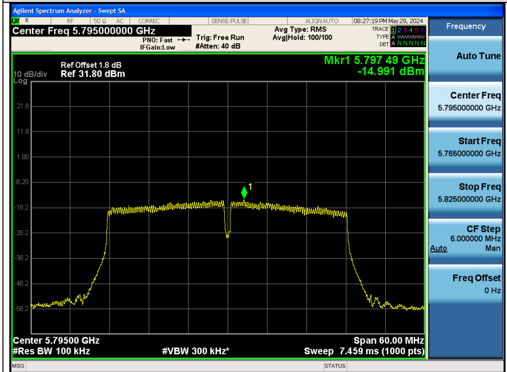
Test_Graph_802.11n40_Chain B_5795_MCS0_PSD
