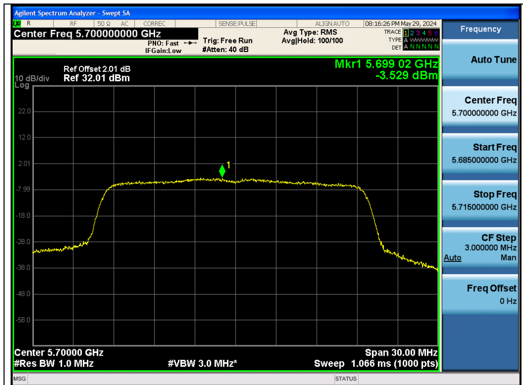
Test_Graph_802.11ax20_Chain B_5700_MCS0_PSD
