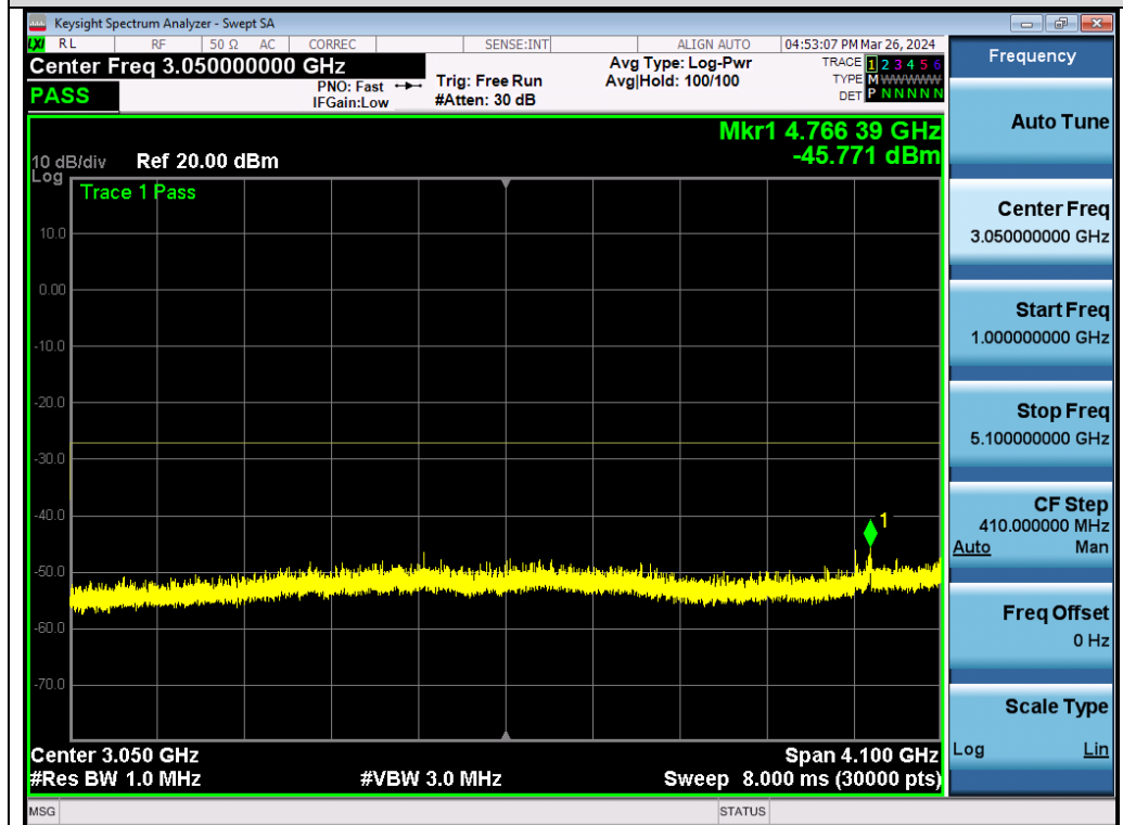
Test_Graph_802.11ac80_Chain A_5210_MCS0_Frequency Band 2
