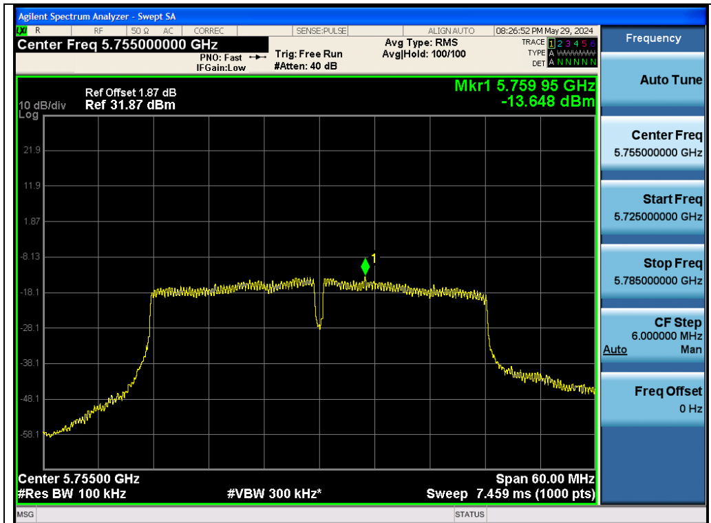
Test_Graph_802.11n40_Chain B_5755_MCS0_PSD
