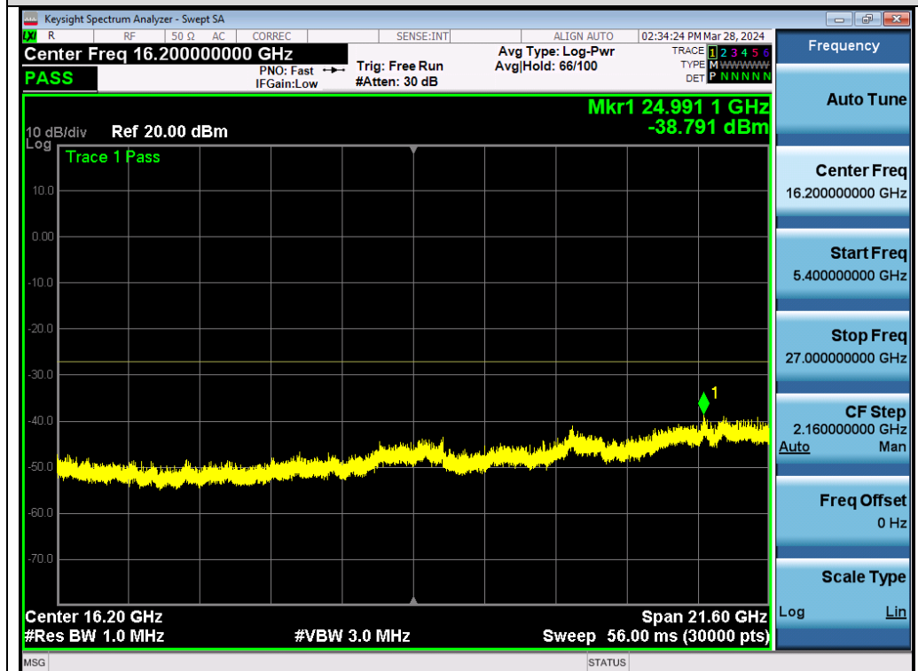
Test_Graph_802.11a_Chain B_5240_6Mbps_Frequency Band 4
