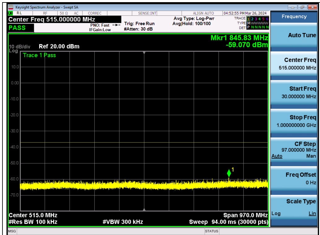
Test_Graph_802.11ac80_Chain A_5210_MCS0_Frequency Band 1
