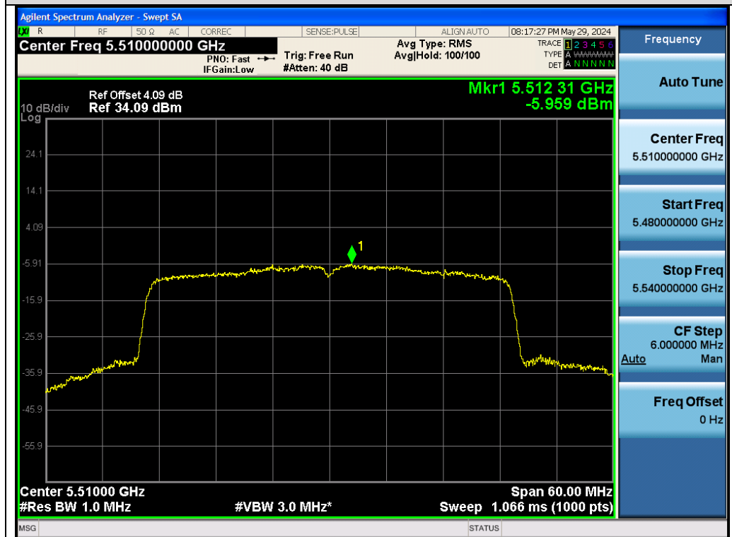
Test_Graph_802.11ax40_Chain B_5510_MCS0_PSD
