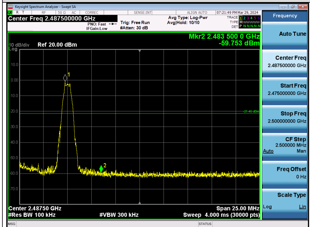
Test_Graph_LE1M_Chain A_2480_1Mbps_Higher Band Edge Emissions
