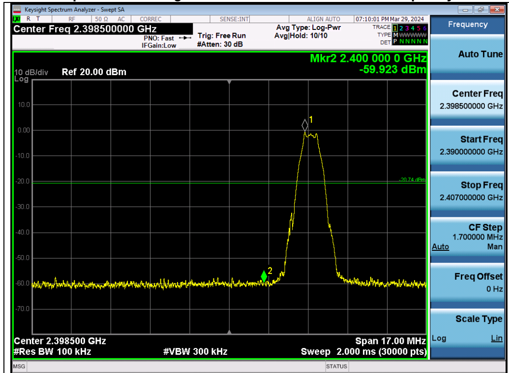
Test_Graph_LE1M_Chain A_2402_1Mbps_Lower Band Edge Emissions
