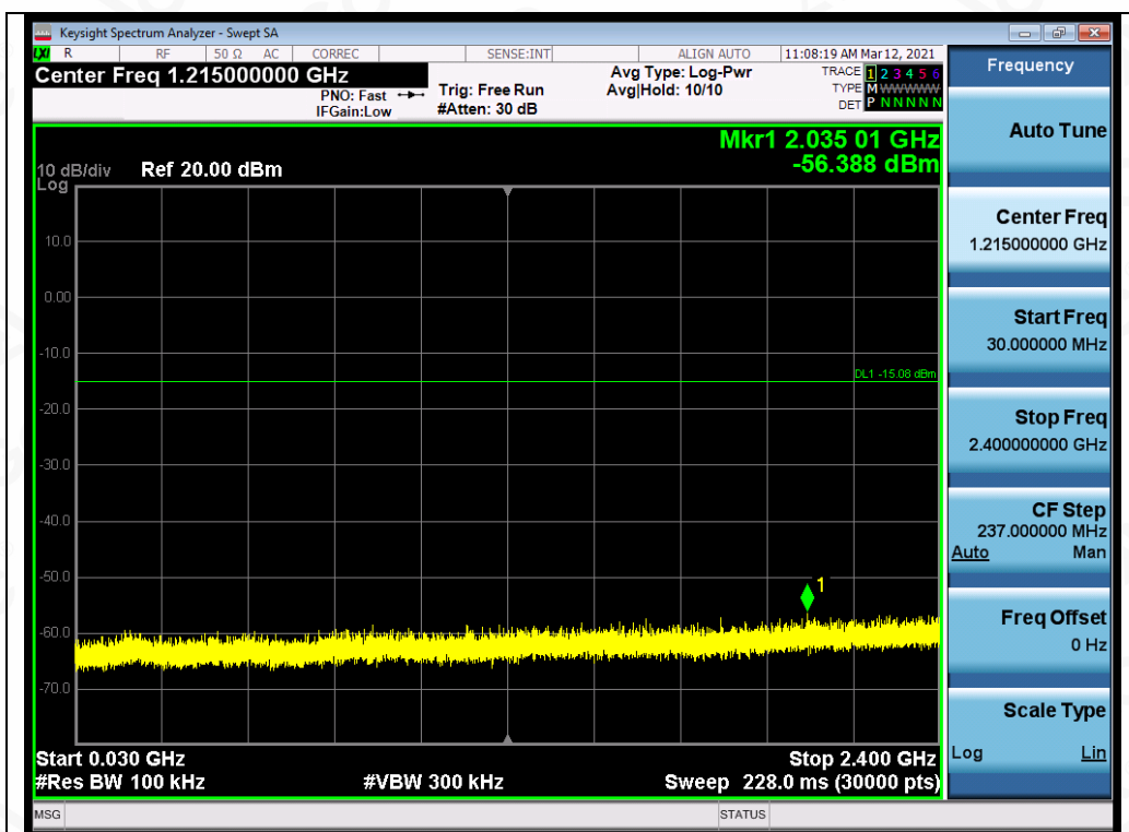
Test_Graph_LE1M_2440_1Mbps_Lower Band Emissions
