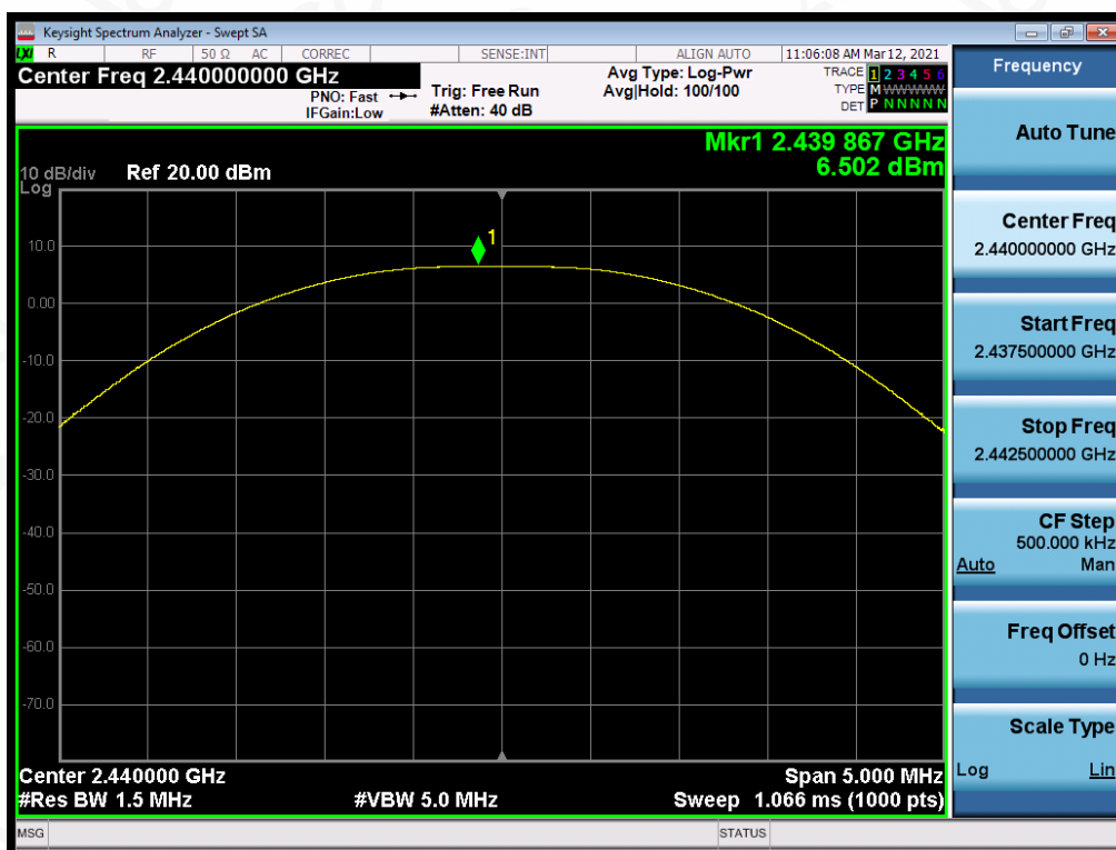
Test_Graph_LE1M_2440_1Mbps_Peak Power
