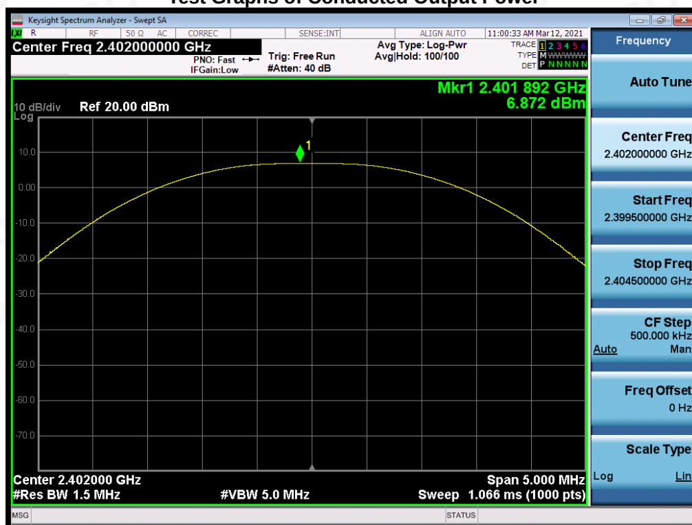
Test_Graph_LE1M_2402_1Mbps_Peak Power
