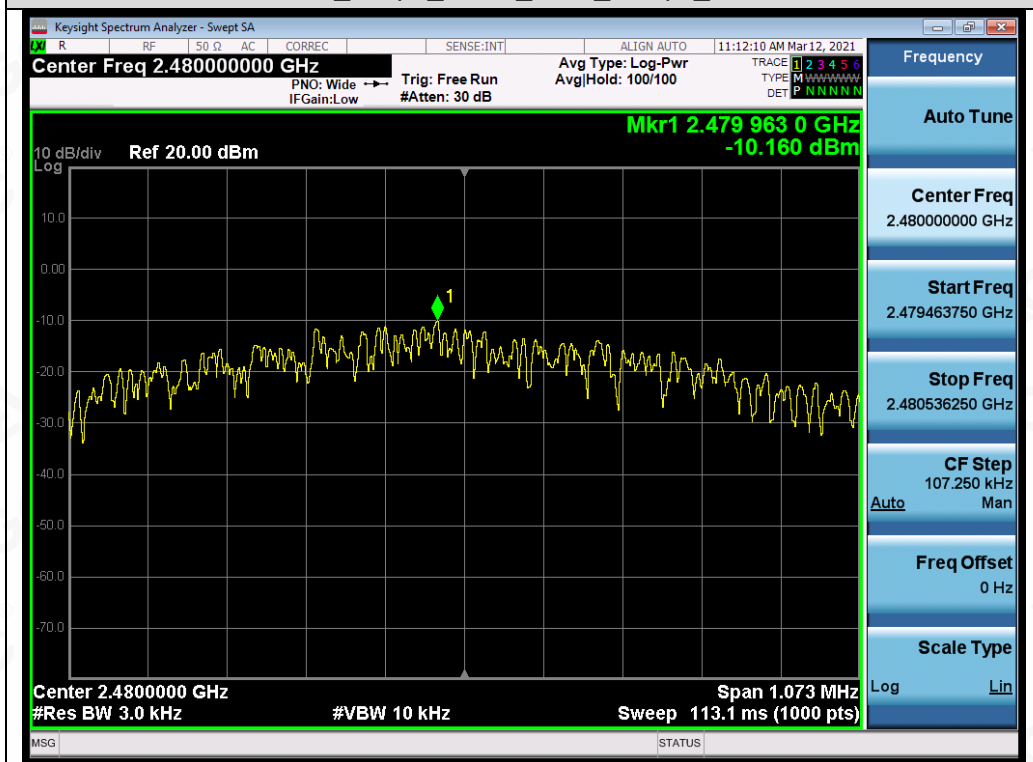
Test_Graph_LE1M_2480_1Mbps_PSD
