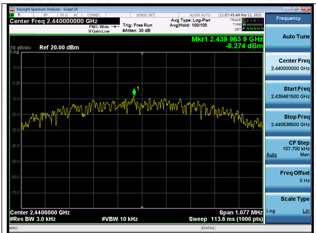
Test_Graph_LE1M_2440_1Mbps_PSD
