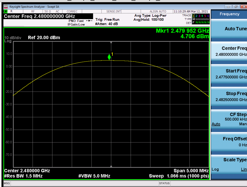
Test_Graph_LE1M_2480_1Mbps_Peak Power
