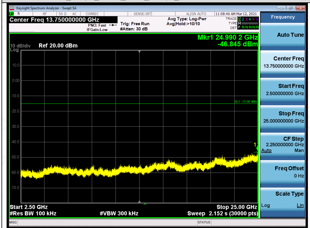
Test_Graph_LE1M_2440_1Mbps_Higher Band Emissions
