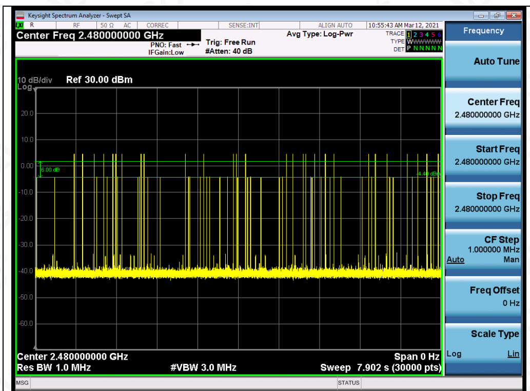
Test_Graph_BR_HOP_NA_1Mbps_2480_Number of Burst
