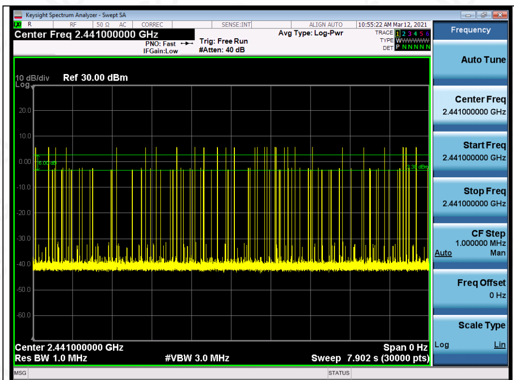
Test_Graph_BR_HOP_NA_1Mbps_2441_Number of Burst
