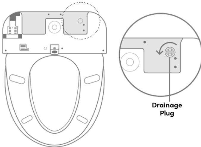
Underside View
