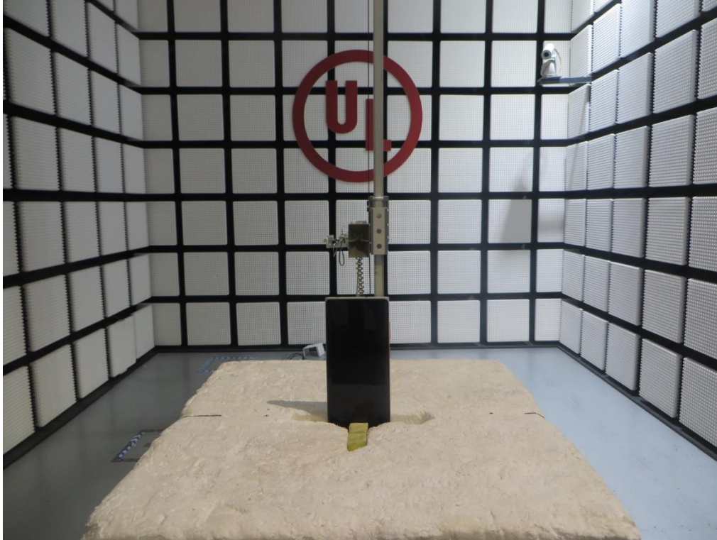
Radiated Band edge and Spurious Emission (Above 1 GHz)
