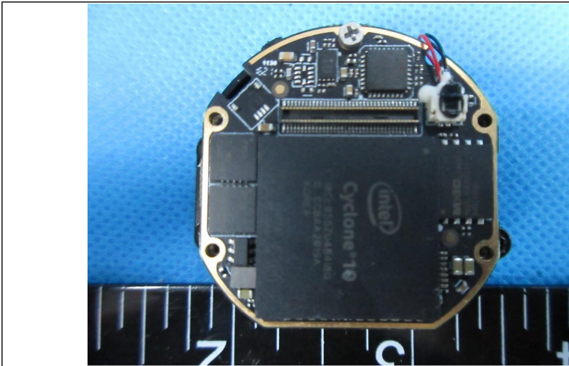
Details of: Internal view 17 of main unit
