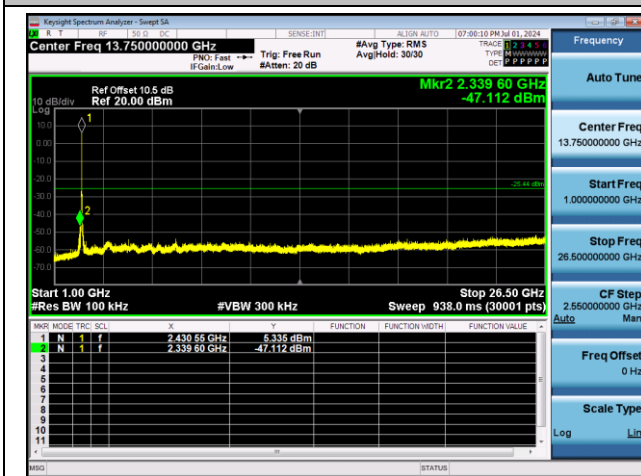
11G-Ant1-2437-1000~26500-PASS
