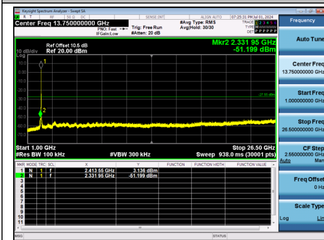
11N20SISO-Ant1-2412-1000~26500-PASS
