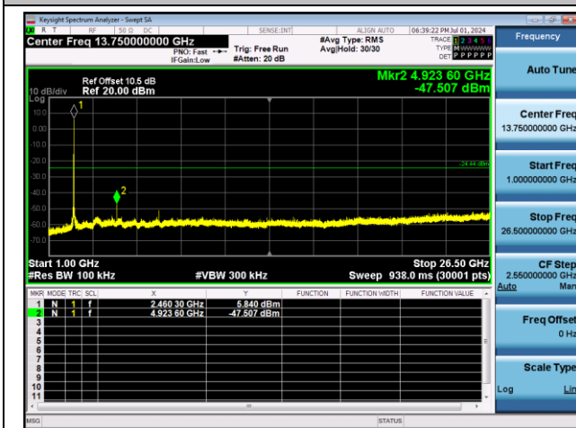
11B-Ant1-2462-1000~26500-PASS
