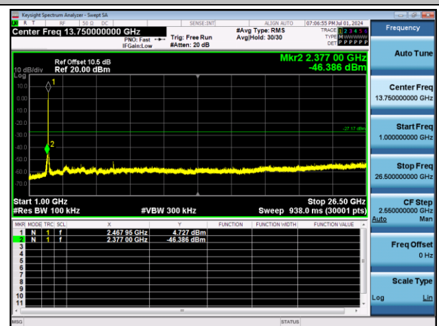
11G-Ant1-2462-1000~26500-PASS
