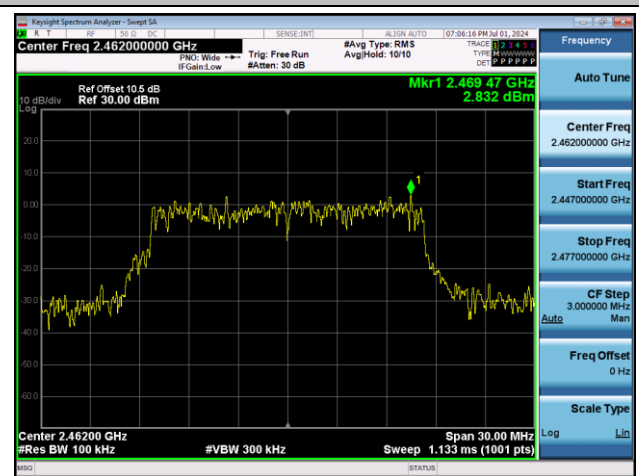
11G-Ant1-2462-0~Reference-PASS
