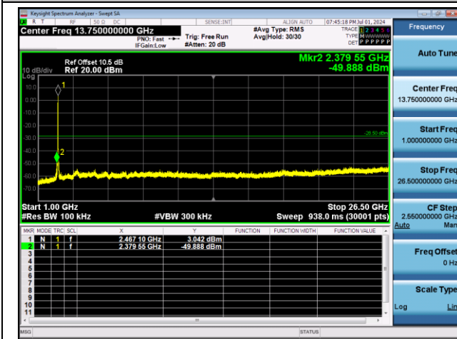
11N20SISO-Ant1-2462-1000~26500-PASS
