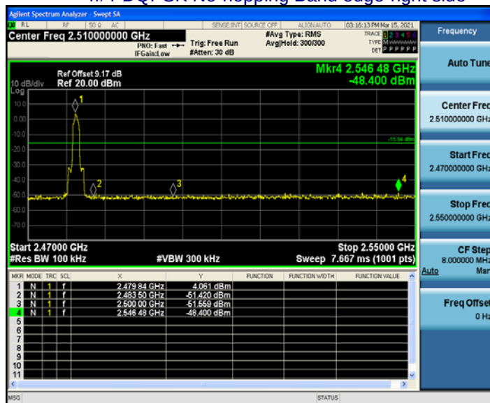
\pi/4 -DQPSK No-hopping Band edge-right side
