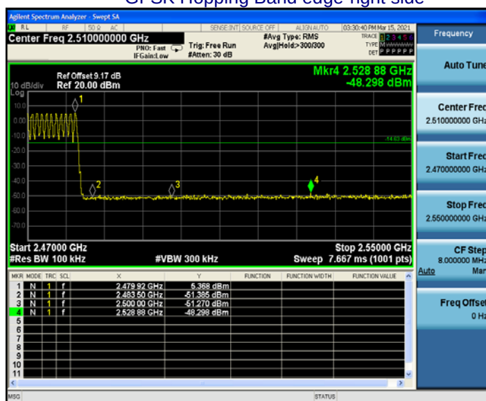
GFSK Hopping Band edge-right side
