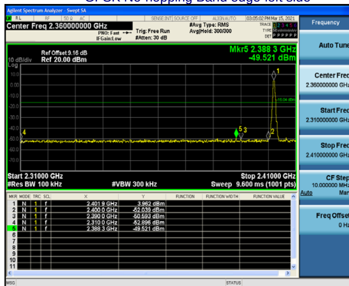
GFSK No-hopping Band edge-left side
