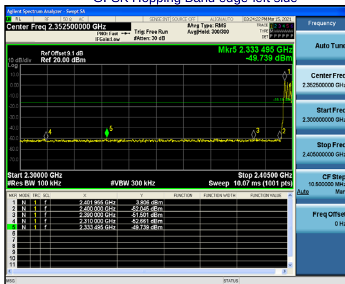
GFSK Hopping Band edge-left side
