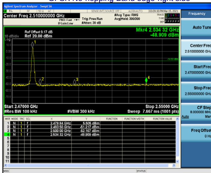
GFSK No-hopping Band edge-right side
