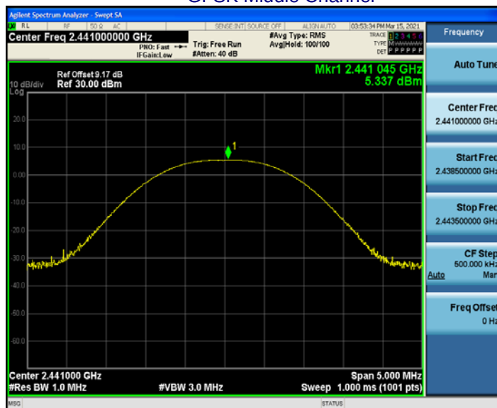
GFSK Middle Channel
