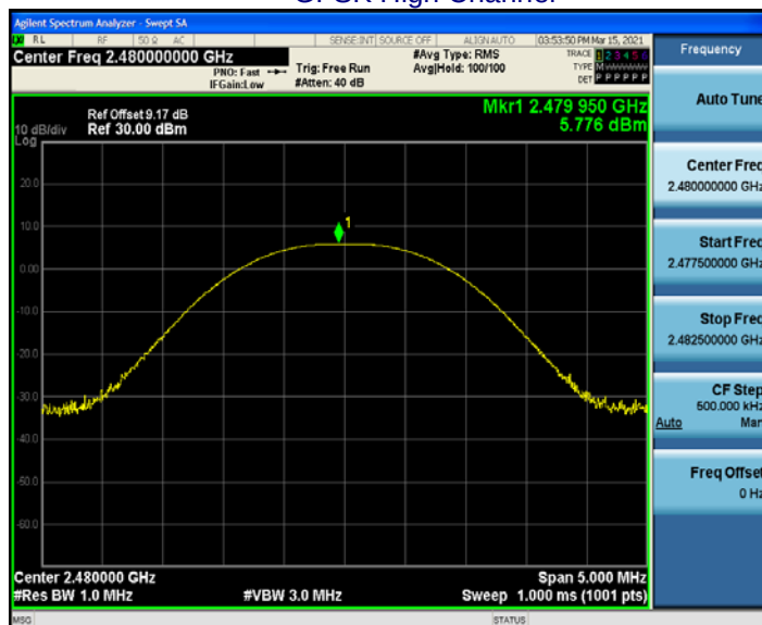
GFSK High Channel
