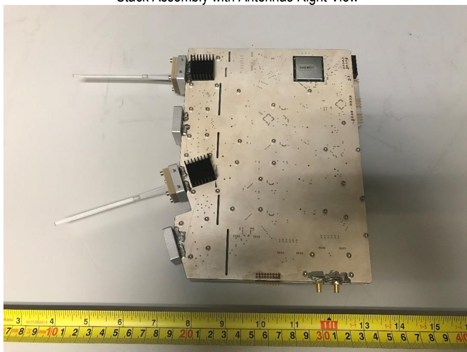
Stack Assembly with Antennas Right View
