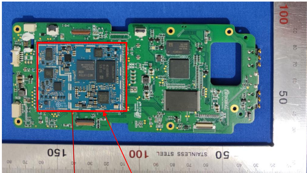
WiFi Chip
