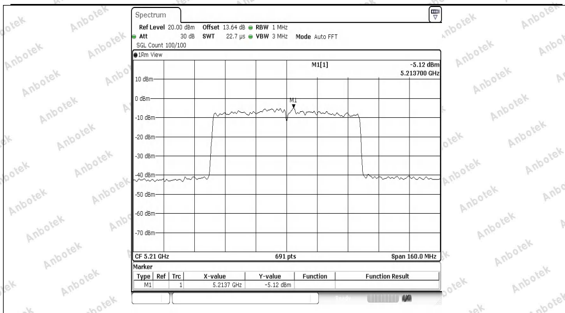
11AC80MIMO-Ant1-5210-PASS
