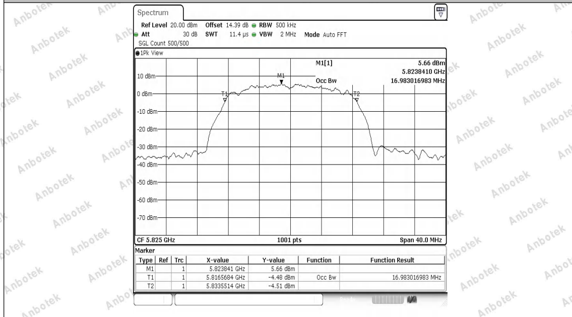
11A-Ant2-5825
