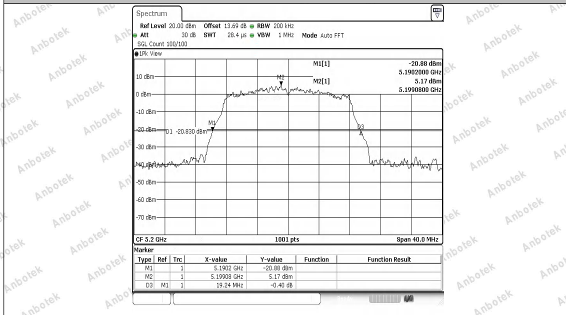
11A-Ant2-5200
