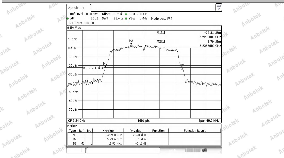
11N20MIMO-Ant2-5240
