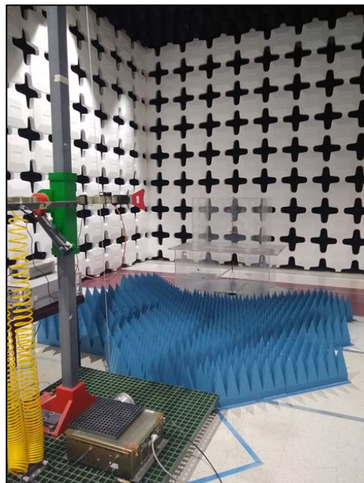
Radiated Spurious Emissions, Setup, 1GHz-18GHz
