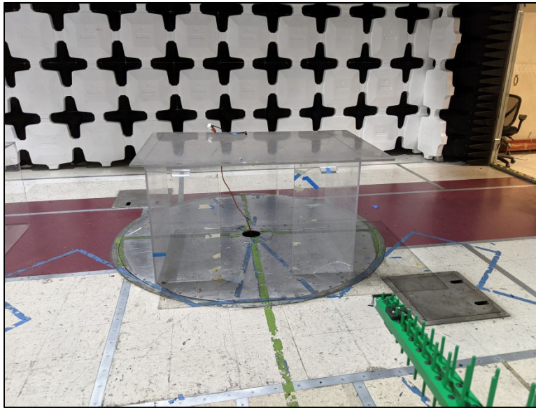
Radiated Spurious Emissions, Setup, 30MHz-1GHz
