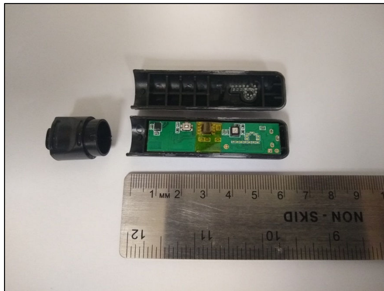
Internal Photo – EUT outer top cover removed
