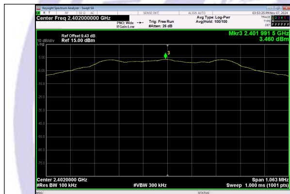
In-Band Reference Level BLE 1M_Channel 0
