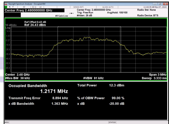
\pi/4 DQPSK_2-DH1_Channel 78
