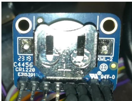
Clock board
