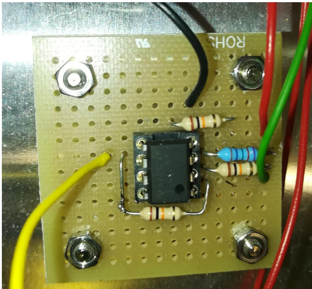
AOP board
