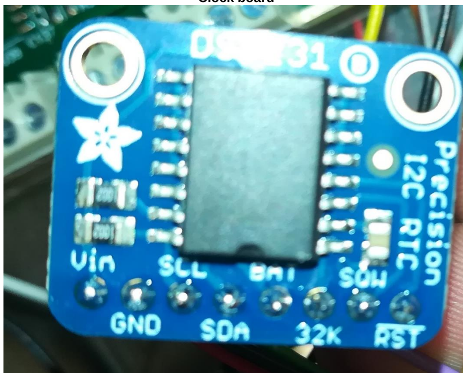
Clock board
