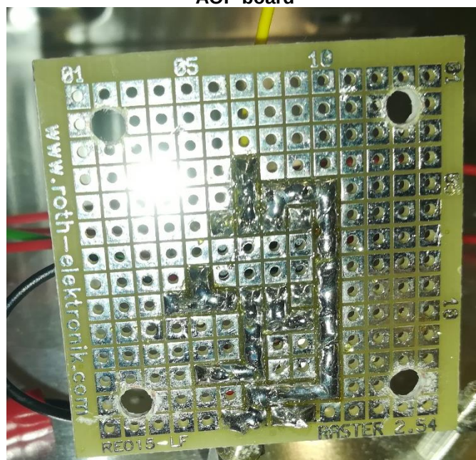
AOP board
