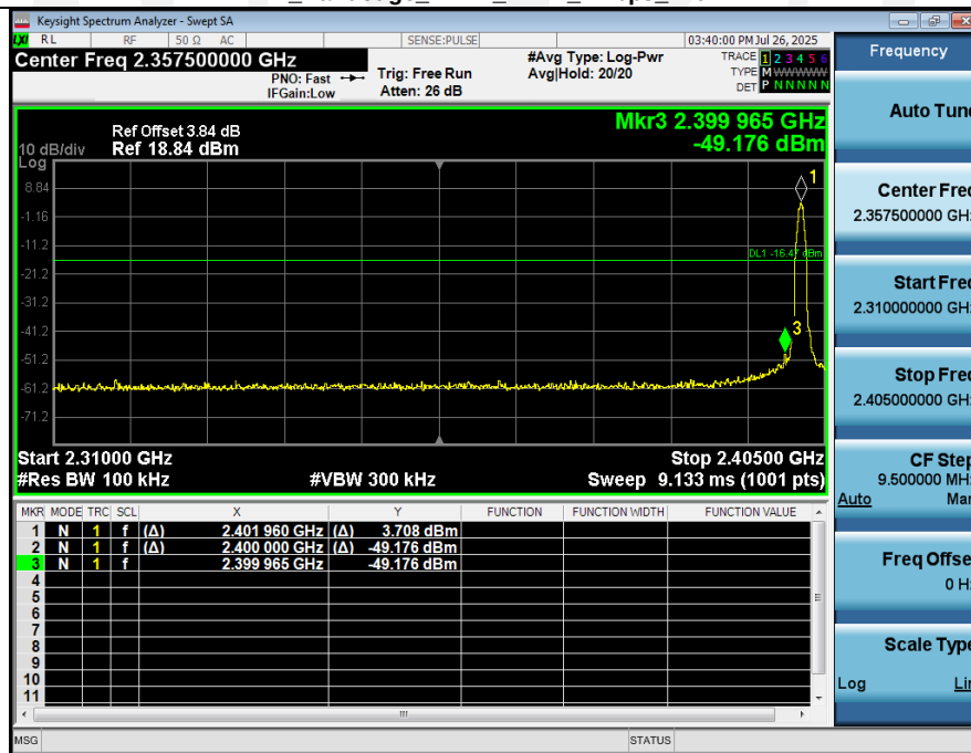
2 Bandedge_NVNT_ANT2_1Mbps_2402
