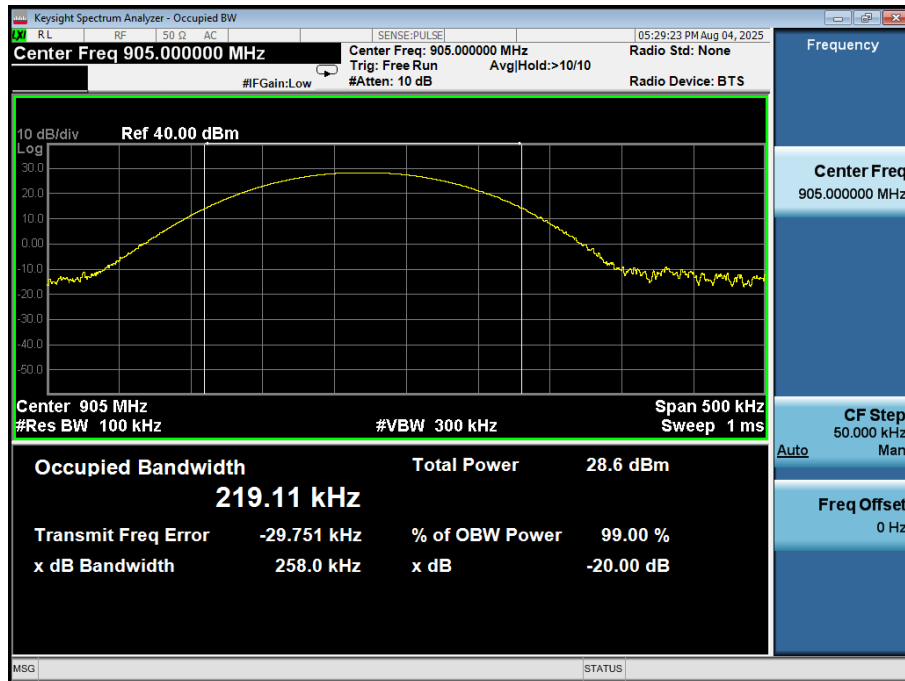
99%_Occupied_Bandwidth_NVNT_ANT1_GFSK_905
