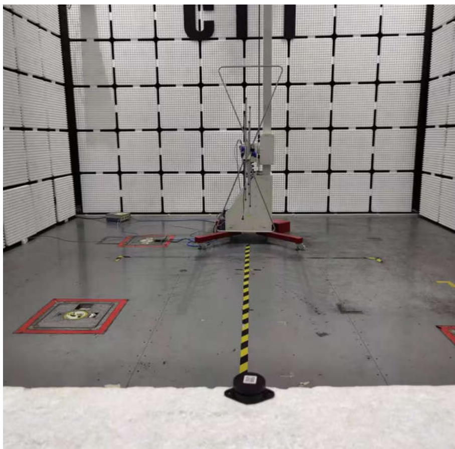
Radiated spurious emission Test Setup-2(Below 1GHz)(close up)
