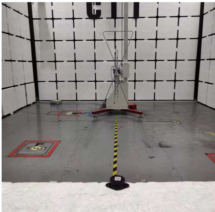
Radiated spurious emission Test Setup-2(Below 1GHz) close up
