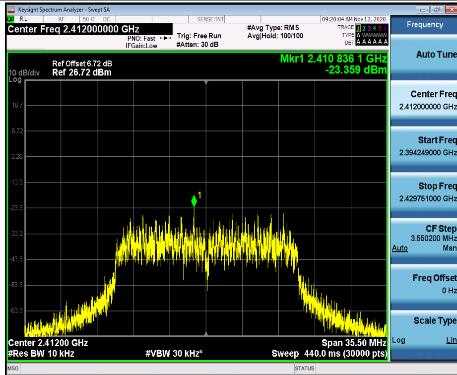
11N20SISO_Ant1_2412
