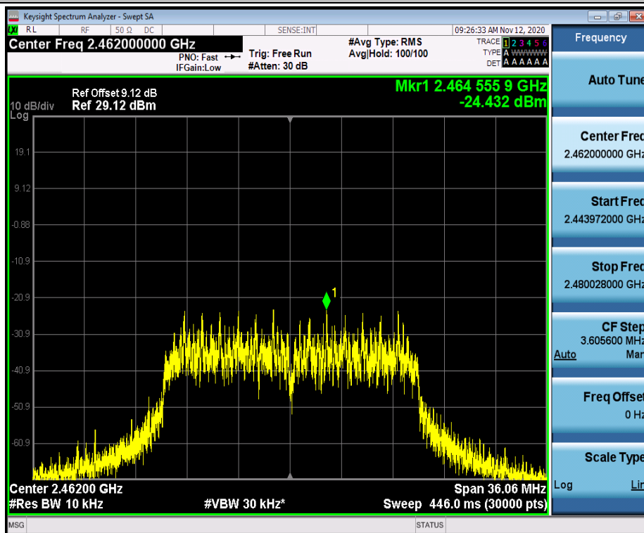
11N20SISO Ant1 2462
