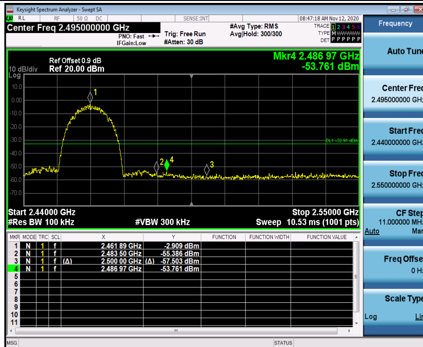
11B_Ant1_High_2462
