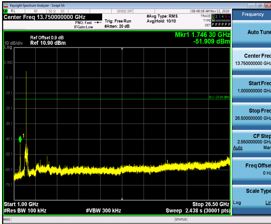
11G_Ant1_2412_0~Reference
