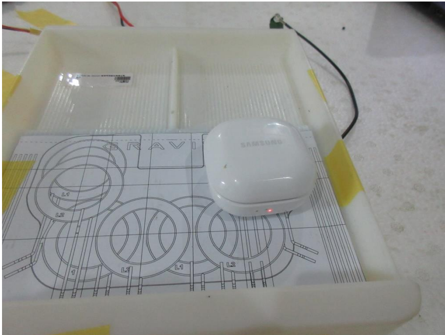
Operating Mode with charging case on Coil 2
