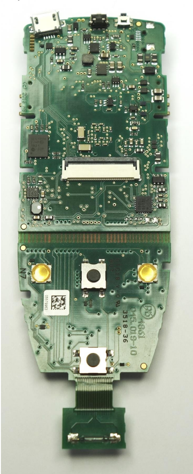
Top view
