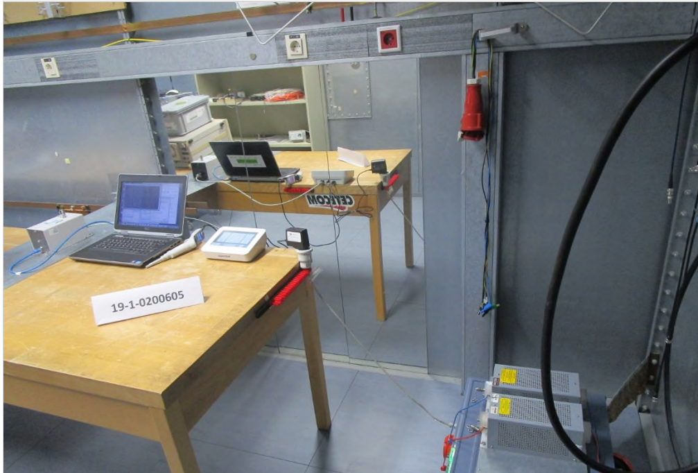
Photograph 1: EUT test setup Conducted emissions on AC-Power lines
