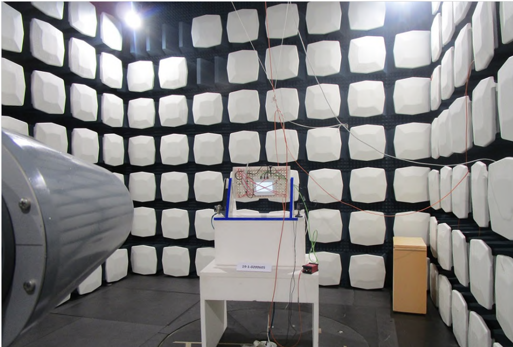
Photograph 5: EUT test setup in the fully anechoic chamber, overview
