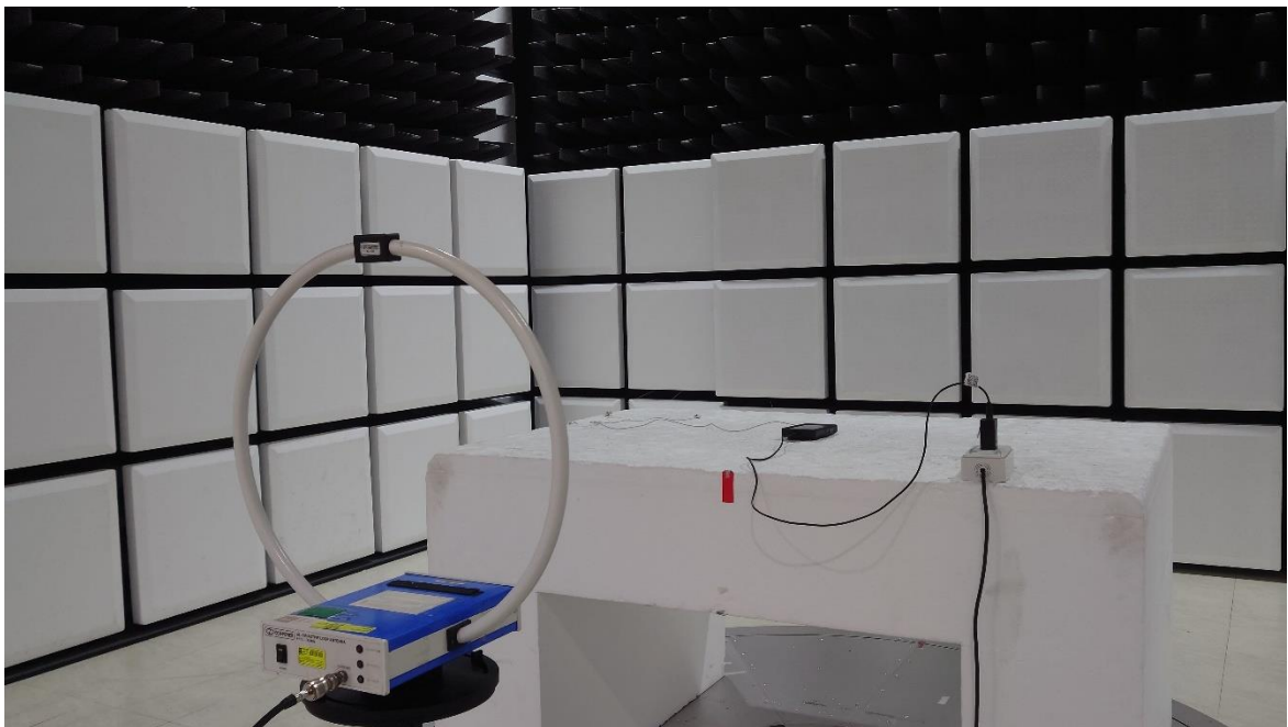
9 kHz ~ 30 MHz _ Rear View
