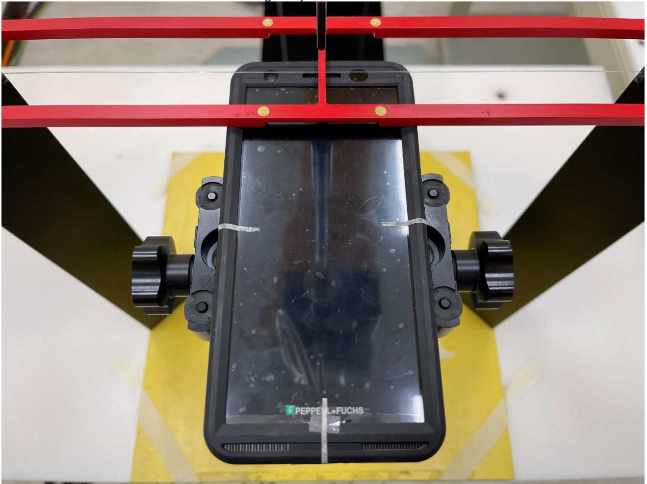
Testing Setup: Front View of DUT
