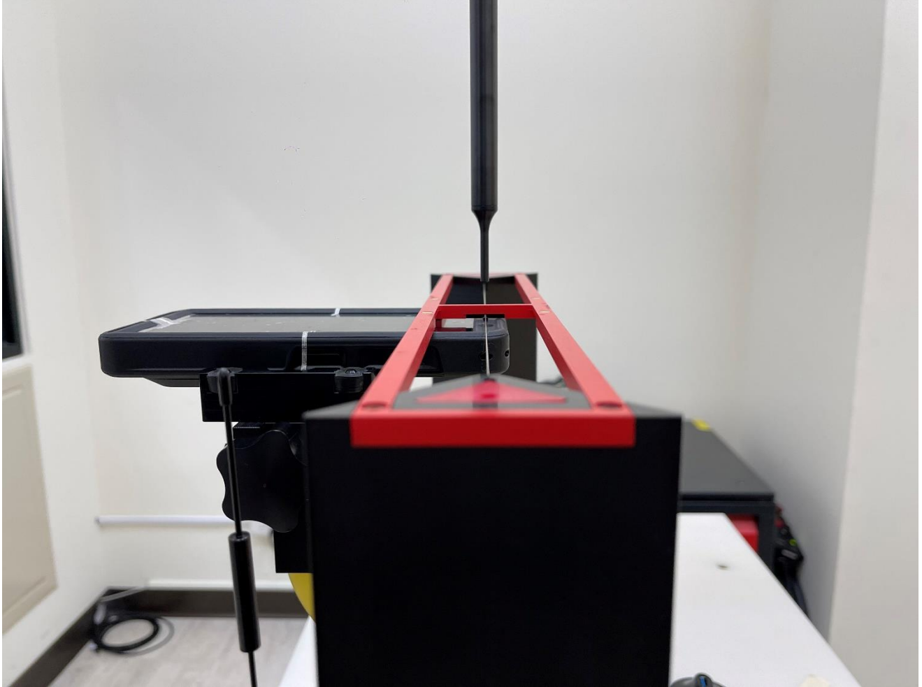
Testing Setup: Ear Reference Point & HAC Phantom Alignment
