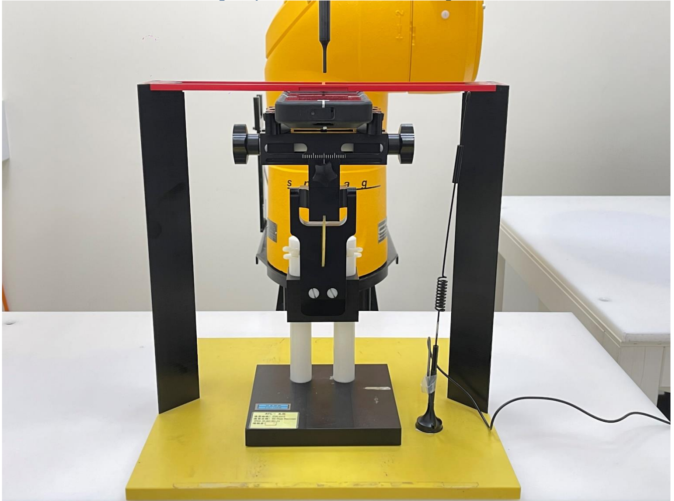
Testing Setup: DUT & HAC Phantom Plane Alignment
