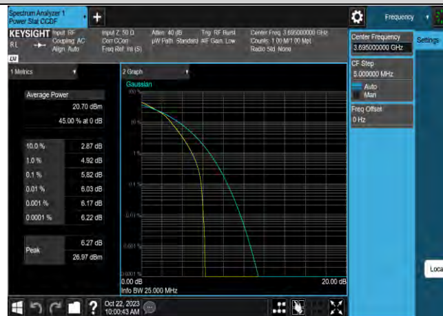
Band48-15MHz-QPSK-55315-1RB#0
