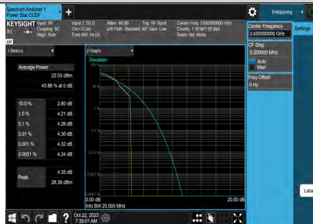
Band43-20MHz-64QAM-44090-100RB#0
