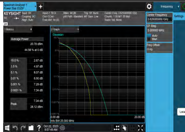
Band48-10MHz-16QAM-56690-1RB#0
