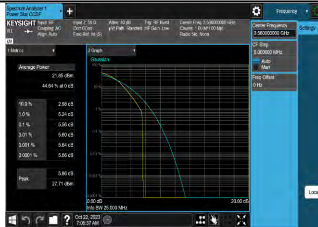
Band42-20MHz-64QAM-43190-100RB#0
