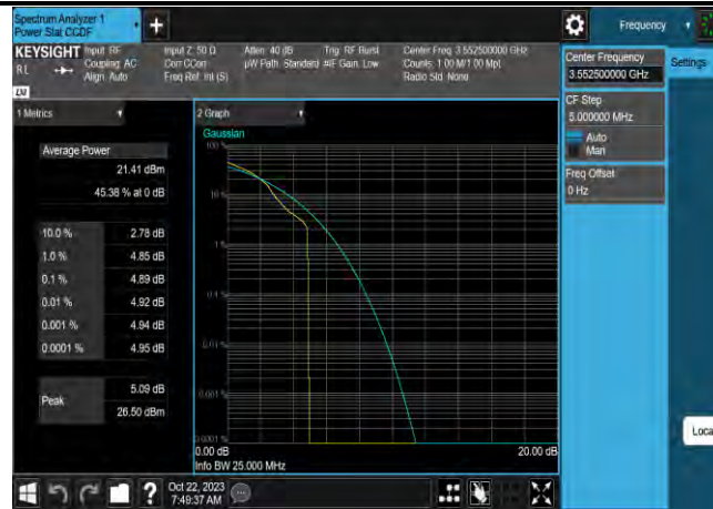
Band48-5MHz-64QAM-55265-25RB#0
