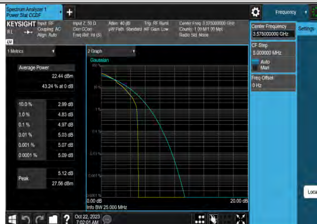
Band42-15MHz-16QAM-43340-75RB#0
