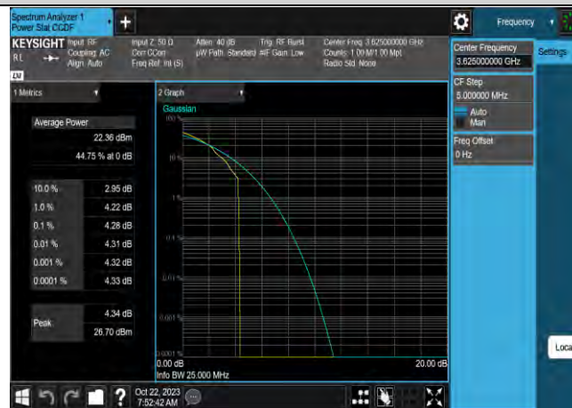
Band48-5MHz-16QAM-55990-25RB#0
