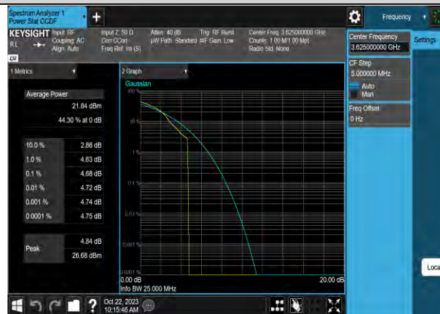
Band48-20MHz-64QAM-55990-100RB#0
