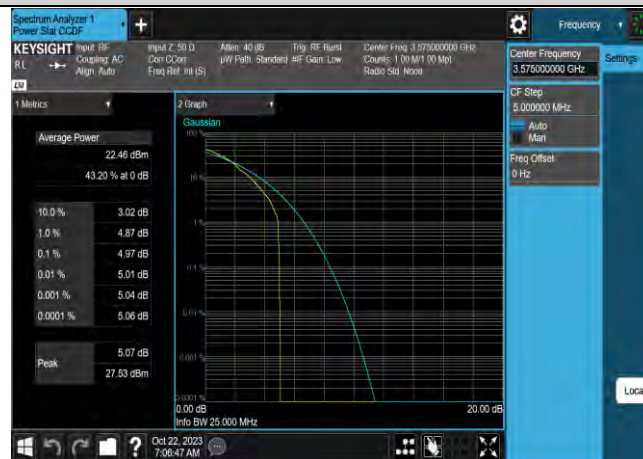
Band42-20MHz-16QAM-43340-100RB#0
