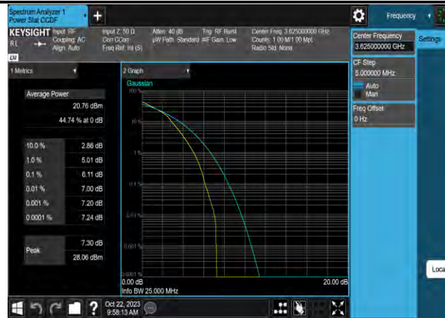
Band48-10MHz-64QAM-56690-1RB#0
