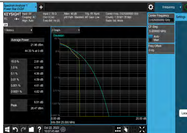
Band48-15MHz-64QAM-55990-75RB#0
