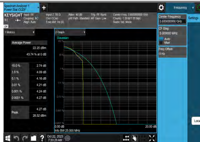
Band43-15MHz-64QAM-44090-75RB#0
