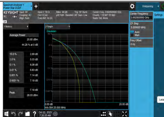
Band43-15MHz-16QAM-43665-1RB#0
