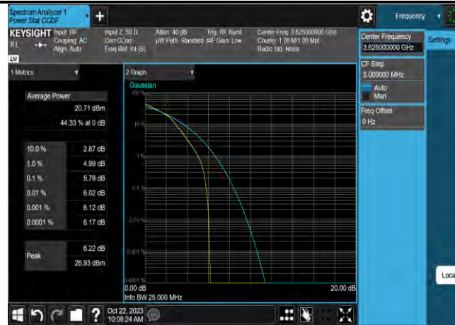
Band48-15MHz-16QAM-56665-1RB#0
