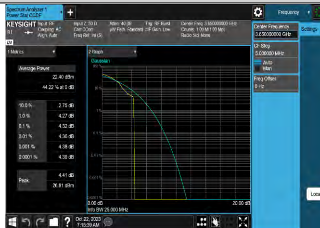
Band43-5MHz-64QAM-44090-25RB#0
