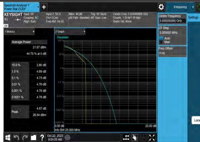
Band48-10MHz-64QAM-55290-50RB#0
