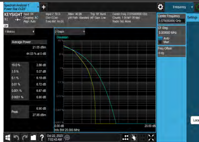
Band42-15MHz-16QAM-43515-1RB#0
