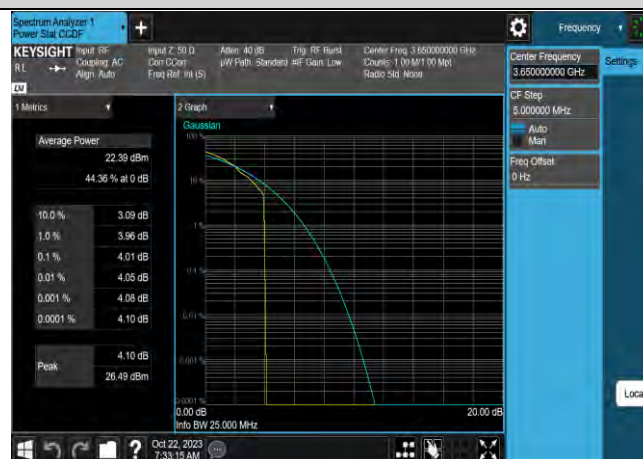
Band43-15MHz-16QAM-44090-75RB#0
