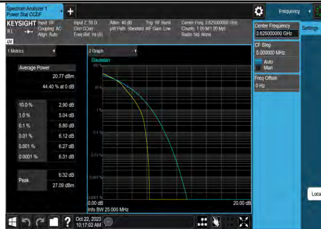
Band48-20MHz-64QAM-56640-1RB#0
