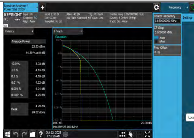
Band43-5MHz-16QAM-44090-25RB#0
