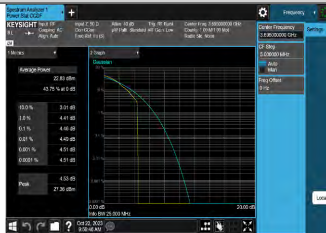
Band48-10MHz-16QAM-56690-50RB#0
