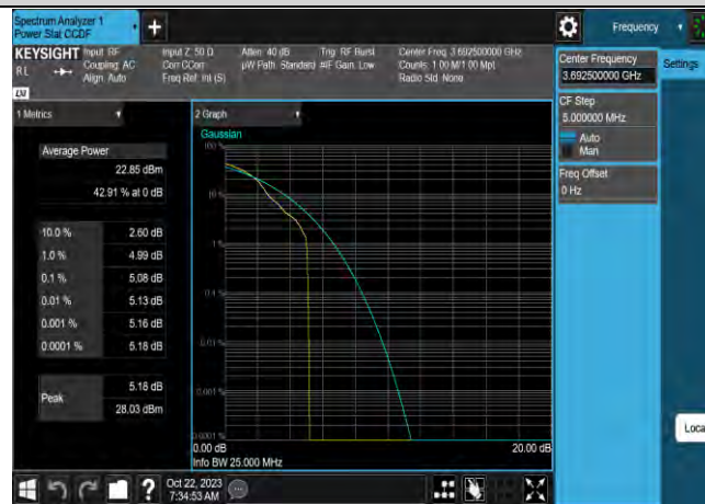
Band43-15MHz-64QAM-44515-75RB#0
