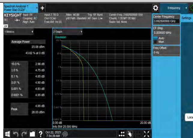
Band43-15MHz-16QAM-44515-75RB#0
