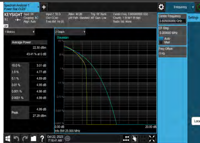
Band43-10MHz-16QAM-43640-50RB#0
