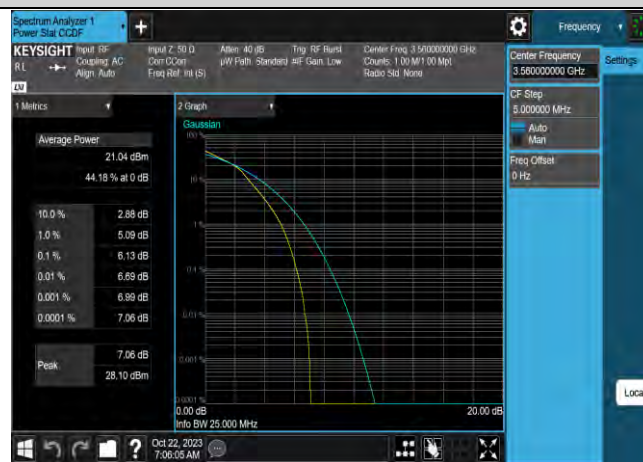
Band42-20MHz-16QAM-43340-1RB#0
