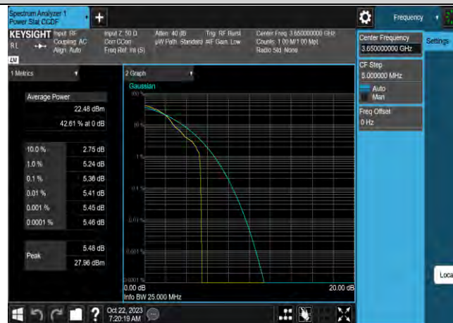
Band43-10MHz-64QAM-44090-50RB#0
