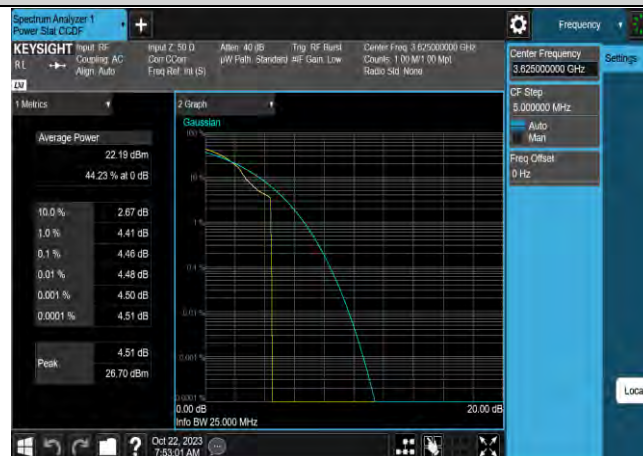
Band48-5MHz-64QAM-55990-25RB#0
