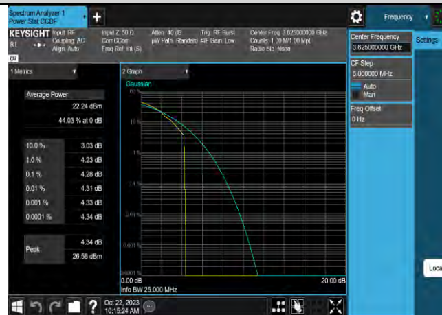
Band48-20MHz-16QAM-55990-100RB#0
