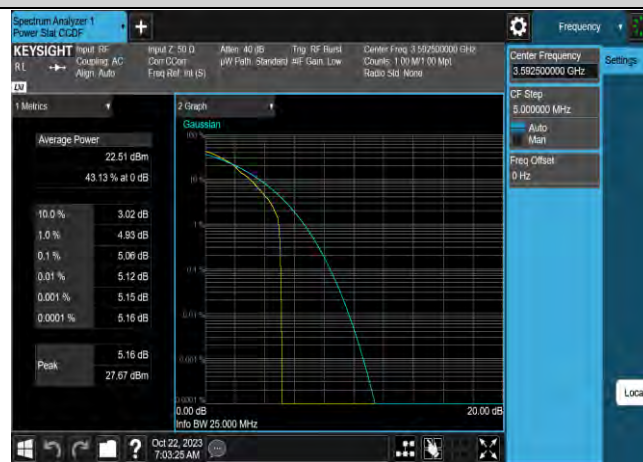
Band42-15MHz-16QAM-43515-75RB#0
