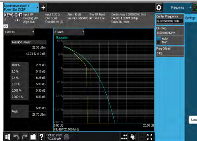
Band42-15MHz-64QAM-43515-75RB#0
