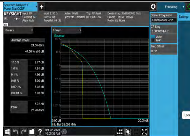
Band48-15MHz-64QAM-55315-75RB#0
