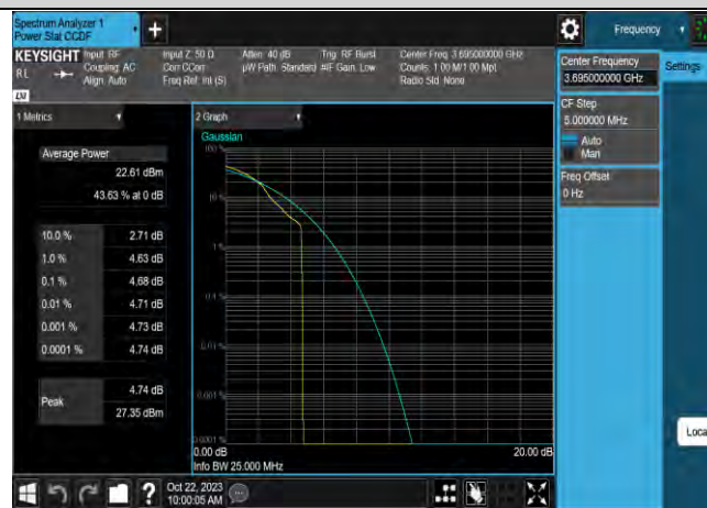
Band48-10MHz-64QAM-56690-50RB#0
