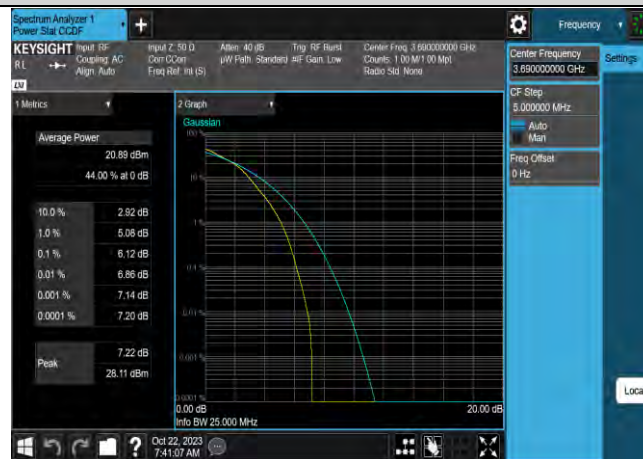
Band43-20MHz-16QAM-43690-1RB#0
