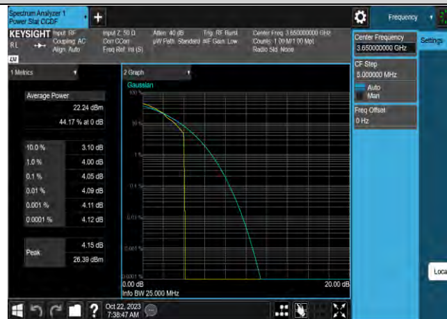
Band43-20MHz-16QAM-44090-100RB#0
