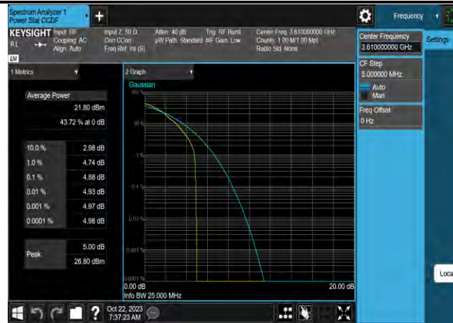
Band43-20MHz-16QAM-43690-100RB#0
