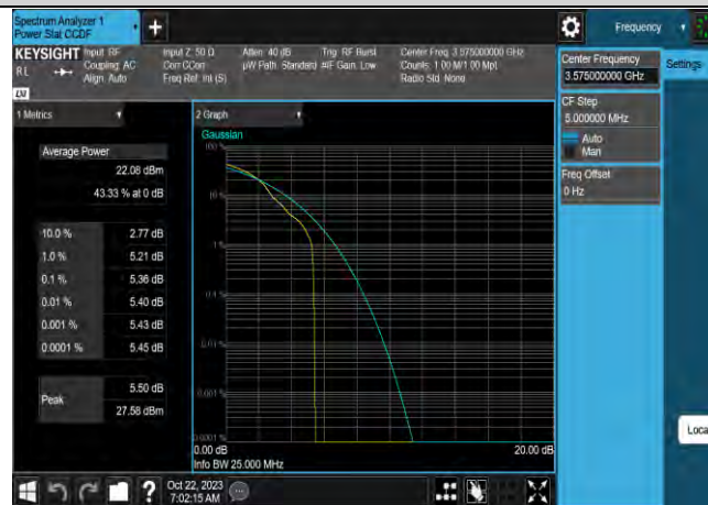
Band42-15MHz-64QAM-43340-75RB#0
