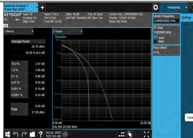
Band48-10MHz-16QAM-55290-1RB#0
