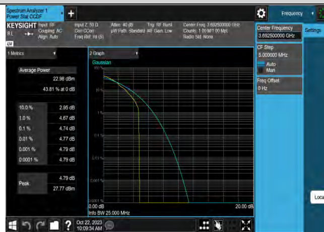
Band48-15MHz-16QAM-56665-75RB#0
