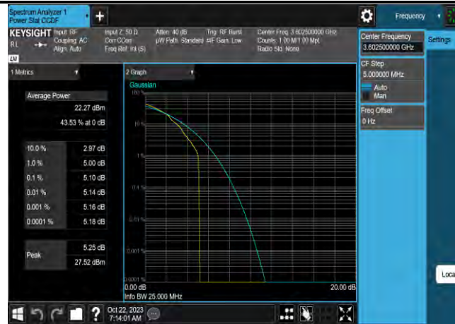
Band43-5MHz-16QAM-43615-25RB#0
