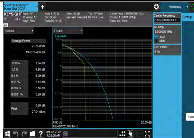
Band43-15MHz-64QAM-43665-75RB#0
