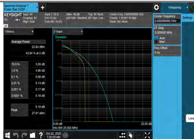
Band43-10MHz-16QAM-44090-50RB#0
