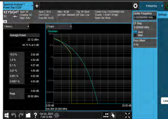
Band48-5MHz-16QAM-55265-25RB#0
