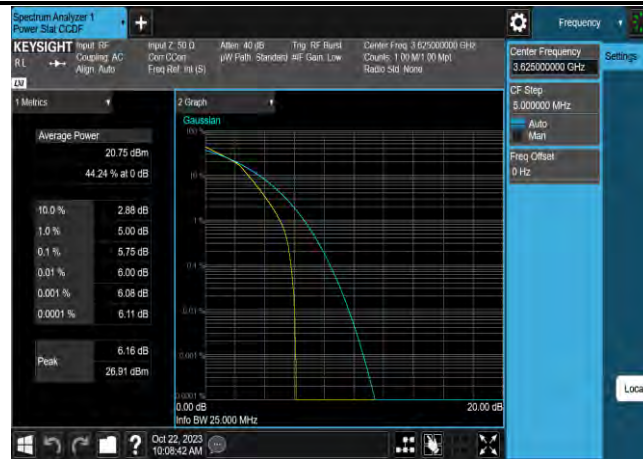
Band48-15MHz-64QAM-56665-1RB#0
