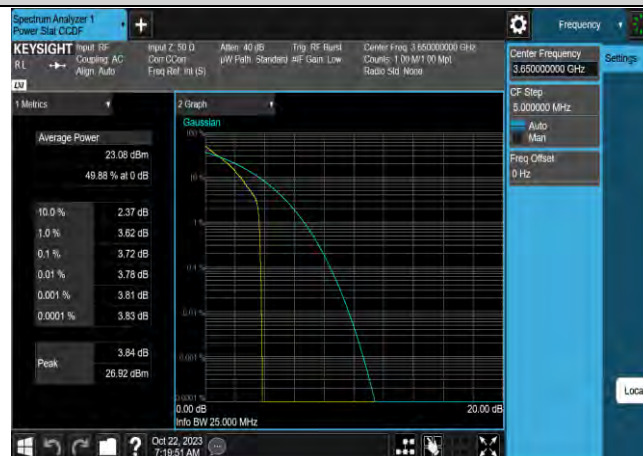
Band43-10MHz-QPSK-44090-50RB#0
