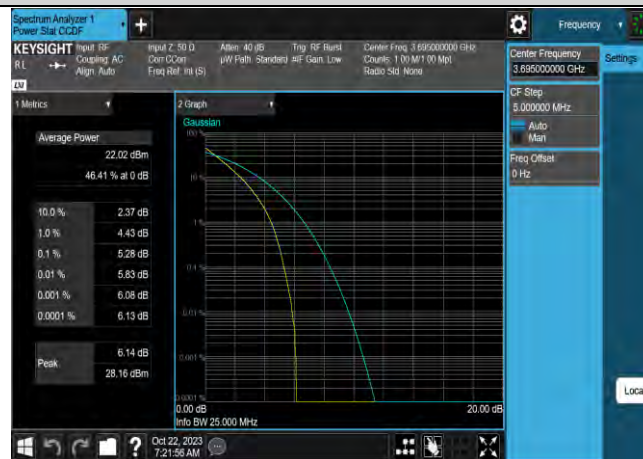
Band43-10MHz-64QAM-43640-1RB#0
