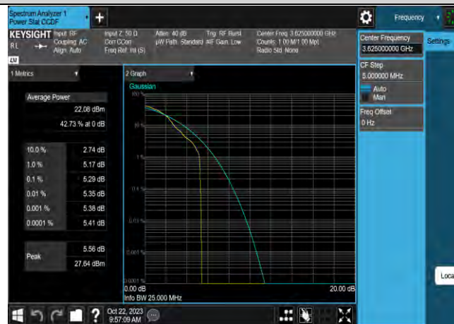
Band48-10MHz-64QAM-55990-50RB#0
