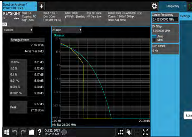
Band42-5MHz-16QAM-42115-25RB#0
