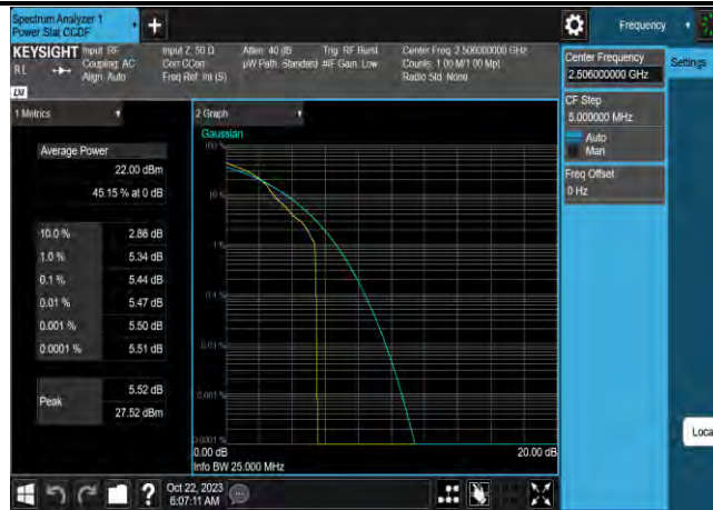
Band41-20MHz-64QAM-39750-100RB#0
