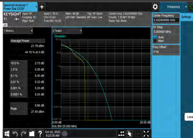
Band42-5MHz-64QAM-42115-25RB#0
