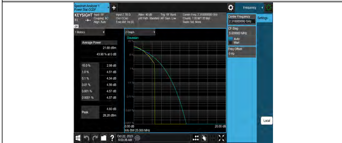
Band40-5MHz-16QAM-38750-25RB#0
