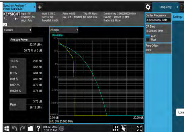
Band42-10MHz-QPSK-42590-50RB#0
