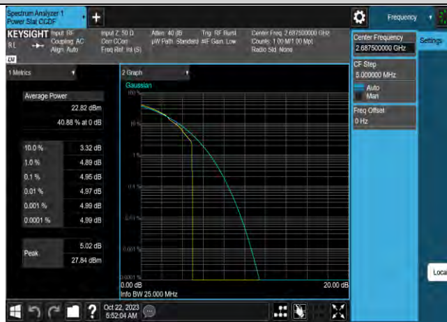
Band41-5MHz-16QAM-41565-25RB#0
