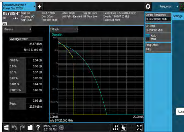
Band42-10MHz-QPSK-43040-50RB#0
