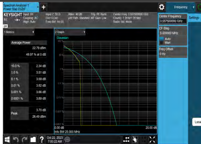
Band42-15MHz-QPSK-43165-75RB#0
