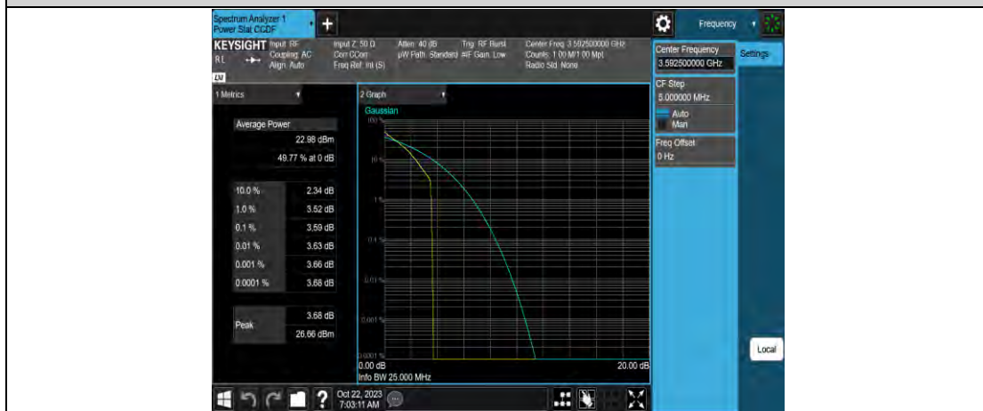
Band42-15MHz-QPSK-43515-75RB#0
