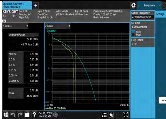
Band41-5MHz-64QAM-39675-25RB#0
