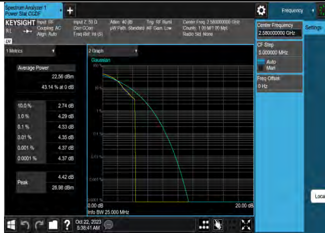
Band38-20MHz-64QAM-37850-100RB#0
