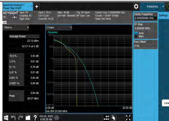
Band41-20MHz-64QAM-40620-100RB#0
