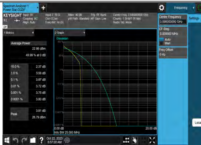
Band42-10MHz-QPSK-43540-50RB#0
