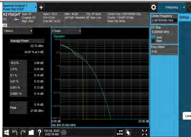
Band41-5MHz-64QAM-41565-25RB#0
