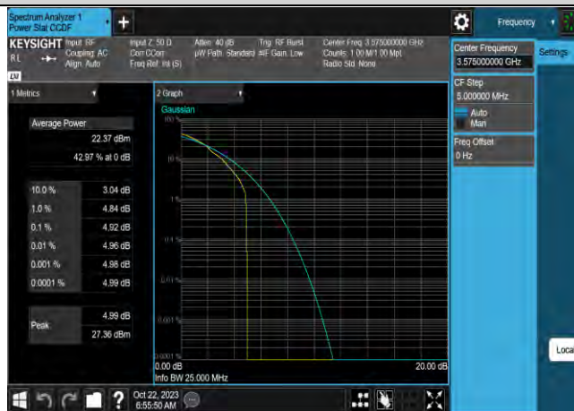
Band42-10MHz-16QAM-43340-50RB#0
