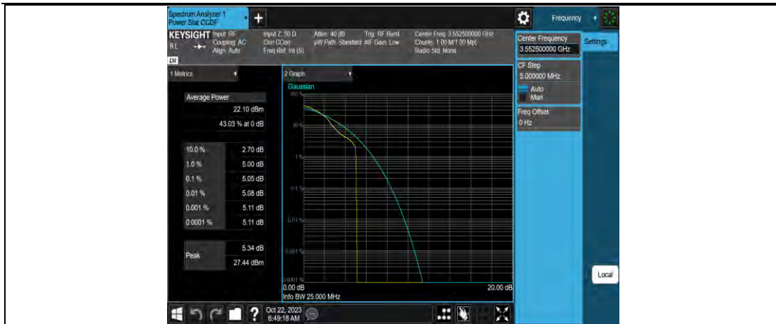
Band42-5MHz-64QAM-43115-25RB#0
