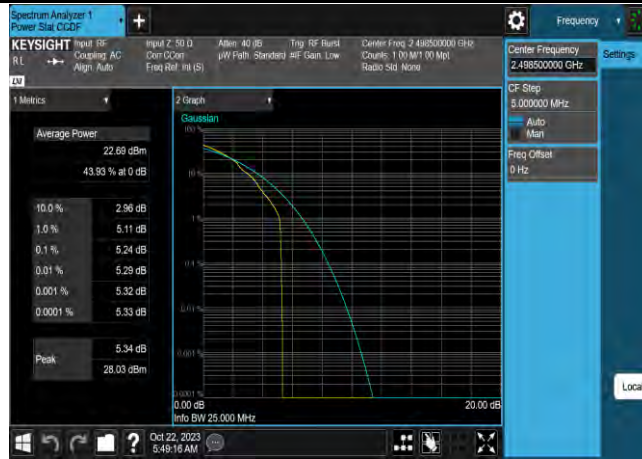
Band41-5MHz-16QAM-39675-25RB#0
