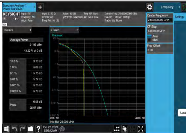
Band41-10MHz-64QAM-40620-50RB#0
