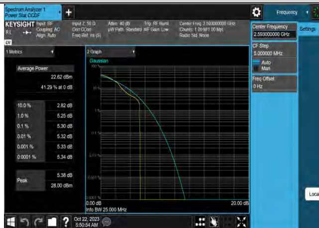
Band41-5MHz-64QAM-40620-25RB#0
