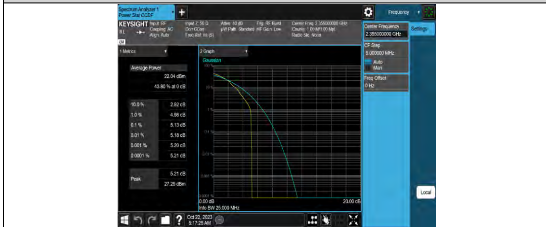
Band40-5MHz-16QAM-39200-25RB#0
