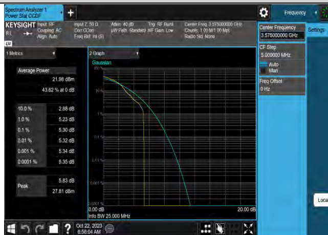
Band42-10MHz-64QAM-43340-50RB#0
