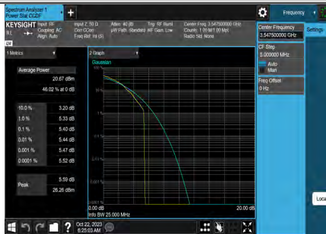
Band42-5MHz-16QAM-43065-25RB#0
