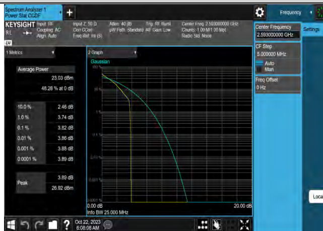
Band41-20MHz-QPSK-40620-100RB#0
