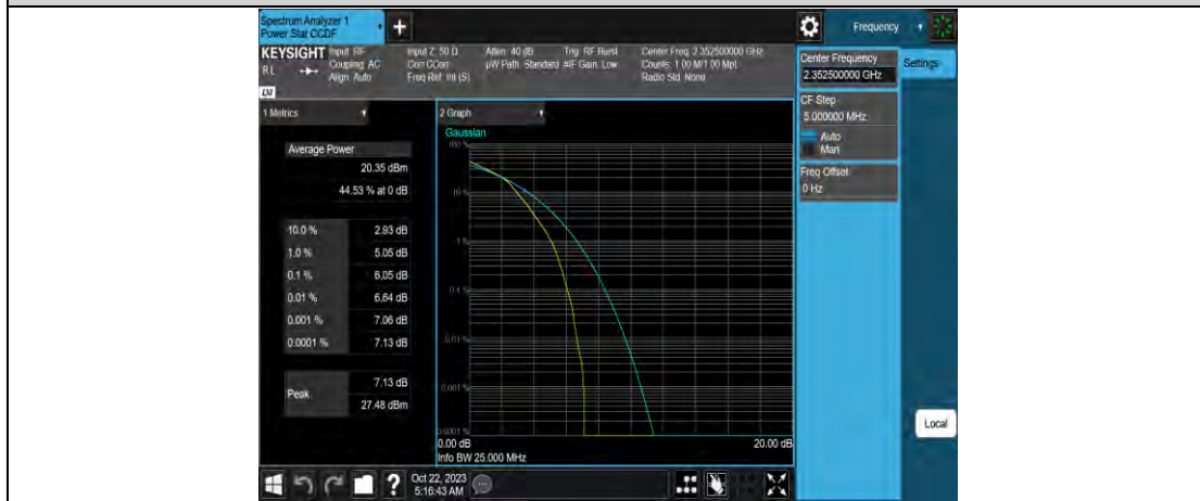
Band40-5MHz-16QAM-39200-1RB#0
