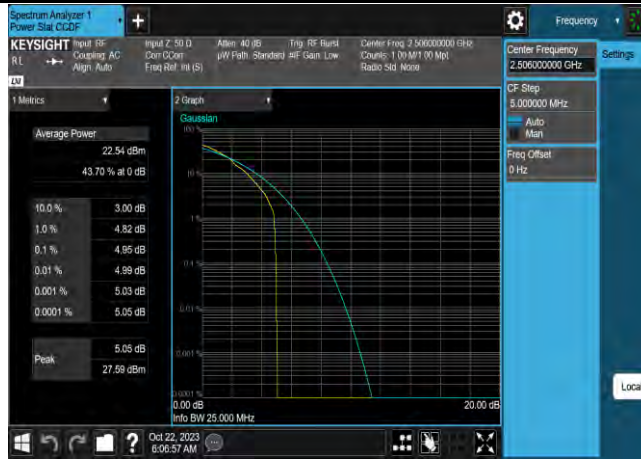
Band41-20MHz-16QAM-39750-100RB#0
