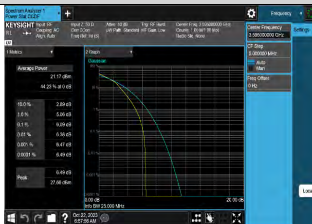
Band42-15MHz-QPSK-43165-1RB#0
