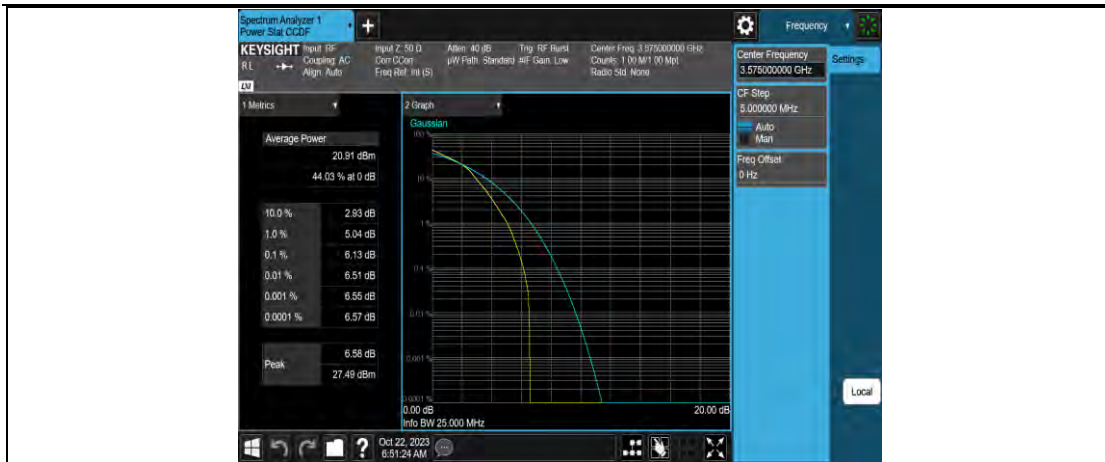
Band42-5MHz-64QAM-43565-1RB#0
