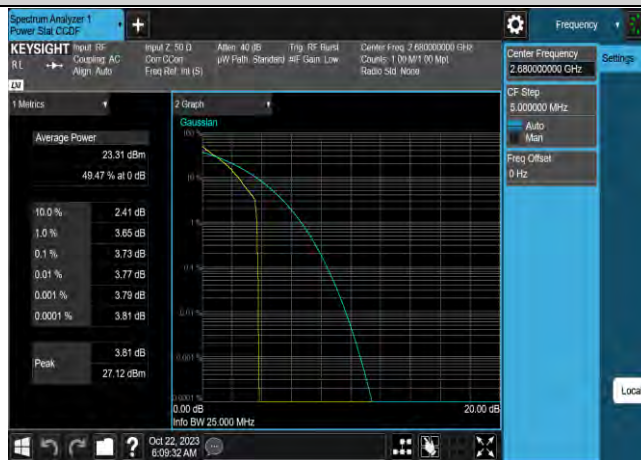
Band41-20MHz-QPSK-41490-100RB#0
