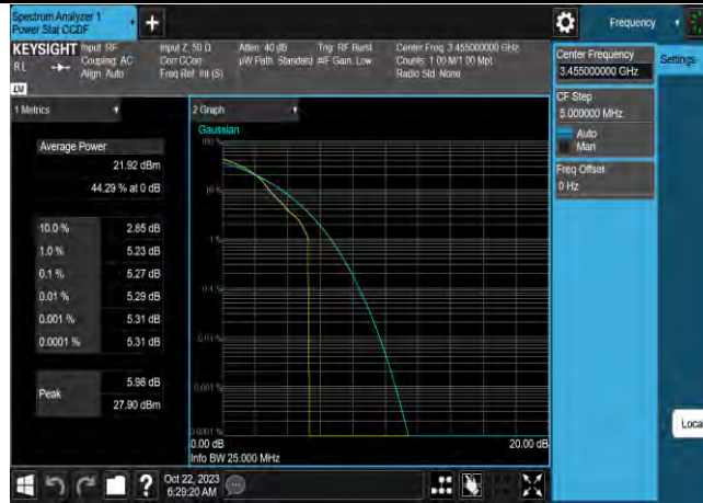
Band42-10MHz-64QAM-42140-50RB#0
