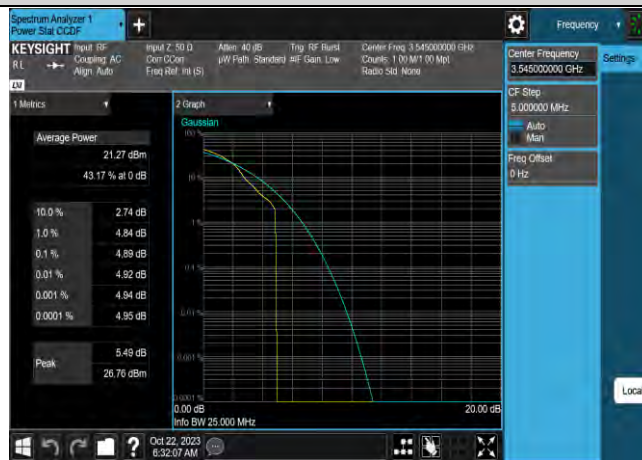
Band42-10MHz-64QAM-43040-50RB#0
