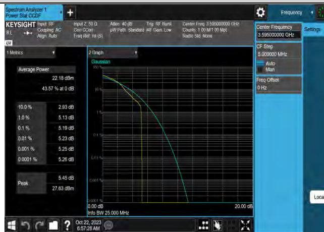
Band42-10MHz-64QAM-43540-50RB#0
