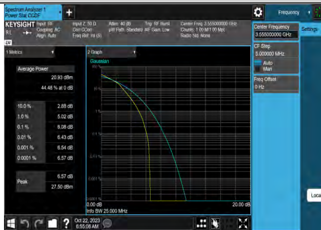
Band42-10MHz-16QAM-43340-1RB#0
