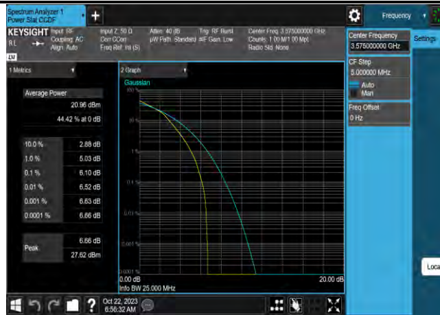
Band42-10MHz-16QAM-43540-1RB#0
