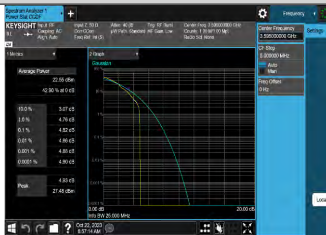
Band42-10MHz-16QAM-43540-50RB#0
