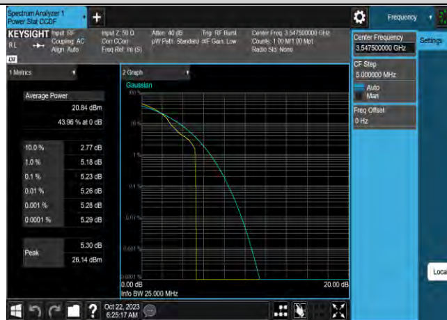
Band42-5MHz-64QAM-43065-25RB#0
