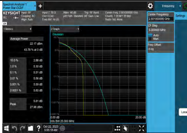
Band41-10MHz-64QAM-39700-50RB#0
