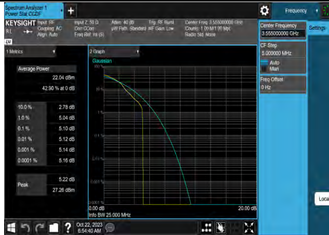
Band42-10MHz-64QAM-43140-50RB#0
