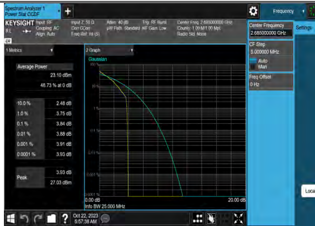
Band41-10MHz-QPSK-41540-50RB#0
