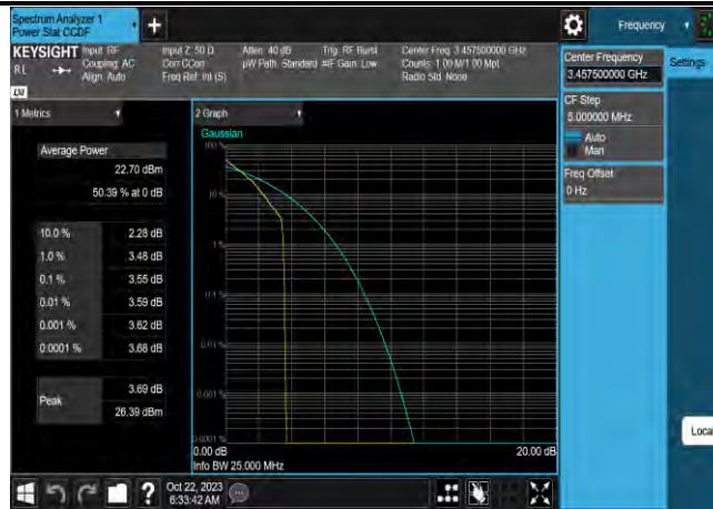
Band42-15MHz-QPSK-42165-75RB#0
