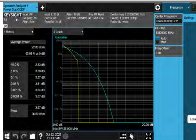
Band42-15MHz-QPSK-43340-75RB#0
