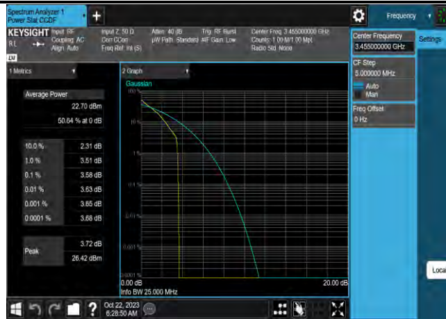
Band42-10MHz-QPSK-42140-50RB#0
