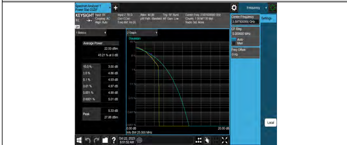
Band42-5MHz-16QAM-43565-25RB#0
