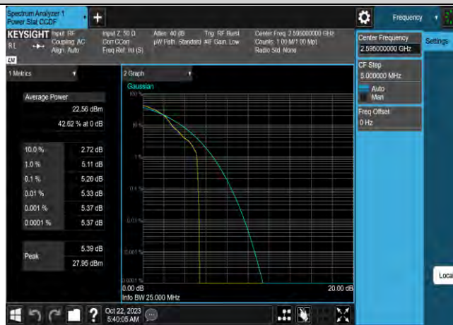
Band38-20MHz-64QAM-38000-100RB#0
