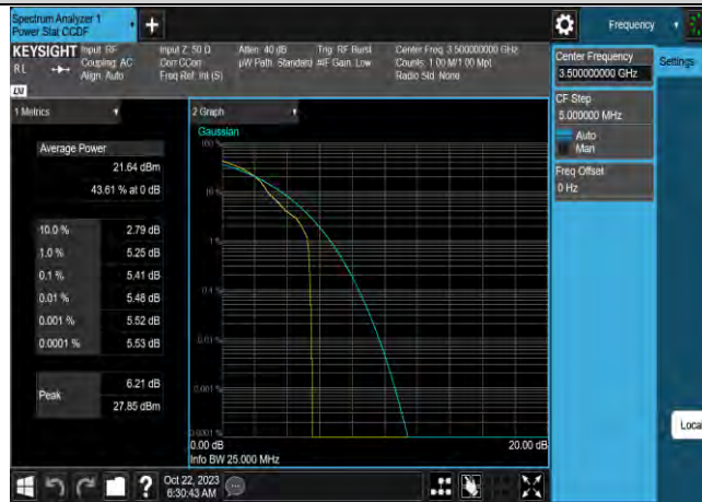
Band42-10MHz-64QAM-42590-50RB#0
