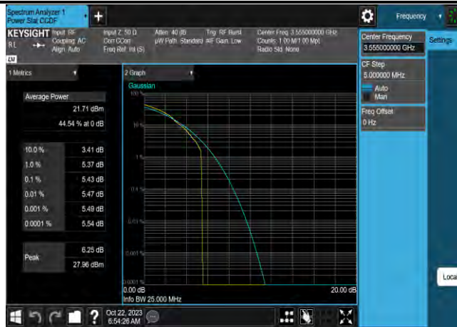
Band42-10MHz-16QAM-43140-50RB#0
