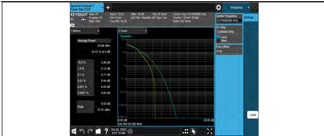
Band42-5MHz-16QAM-43565-1RB#0
