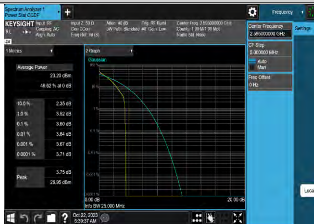
Band38-20MHz-QPSK-38000-100RB#0
