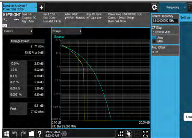
Band42-5MHz-16QAM-42590-25RB#0
