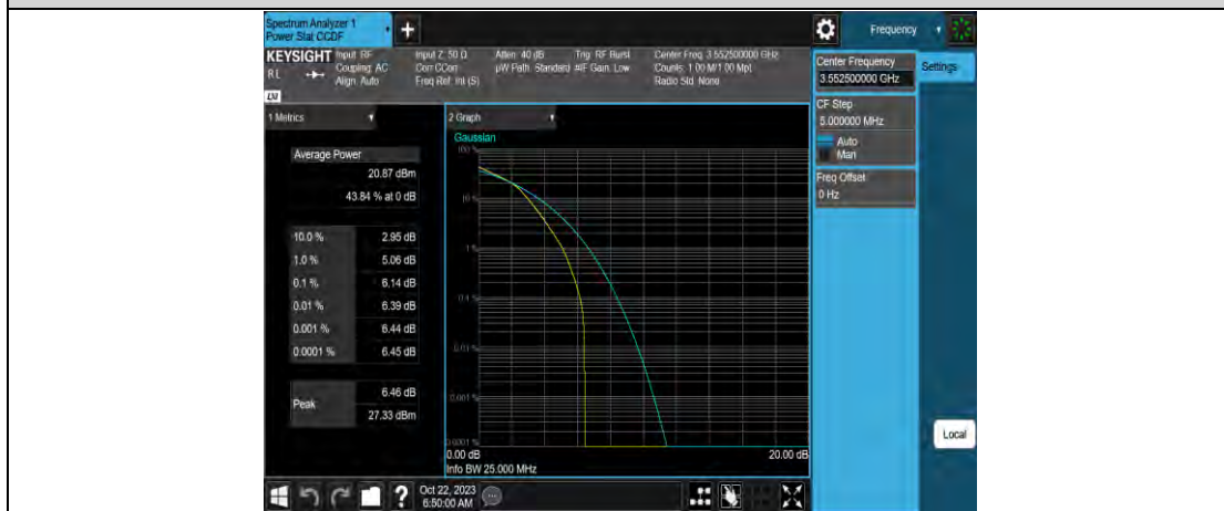
Band42-5MHz-64QAM-43340-1RB#0
