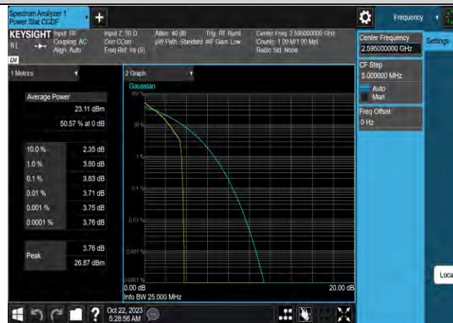
Band38-10MHz-QPSK-38000-50RB#0
