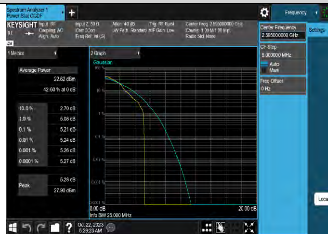
Band38-10MHz-64QAM-38000-50RB#0
