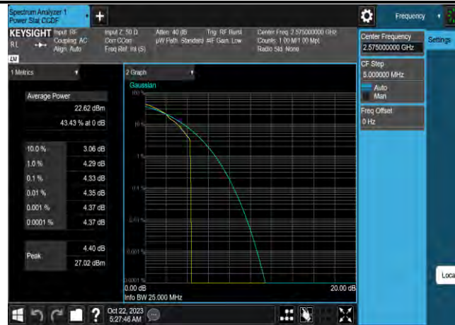
Band38-10MHz-16QAM-37800-50RB#0
