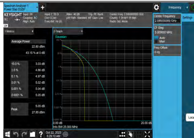
Band38-10MHz-16QAM-38000-50RB#0
