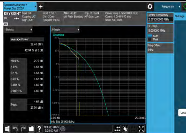
Band38-10MHz-64QAM-37800-50RB#0
