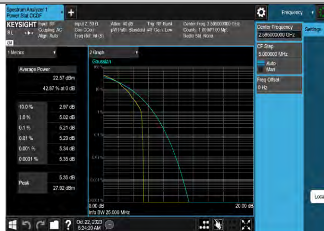
Band38-5MHz-16QAM-38000-25RB#0
