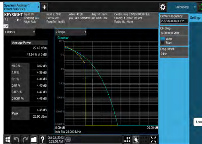
Band38-5MHz-16QAM-37775-25RB#0
