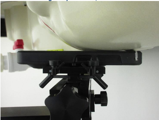
Testing Setup for Head, Left Cheek
