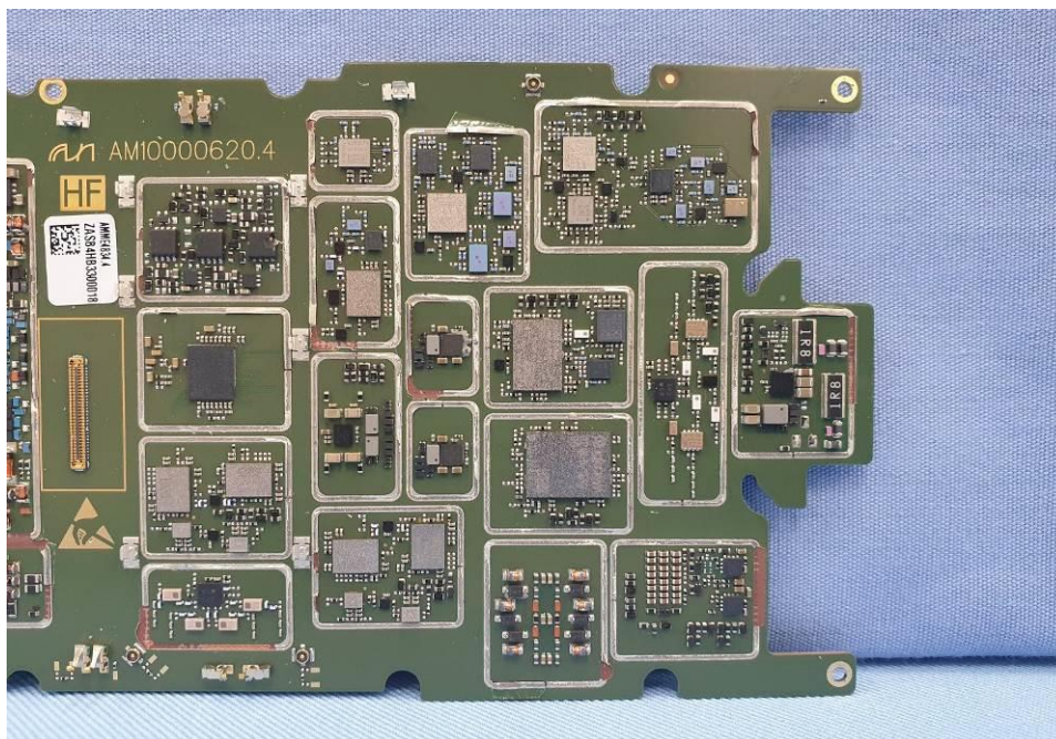
EUT Photo (26)
