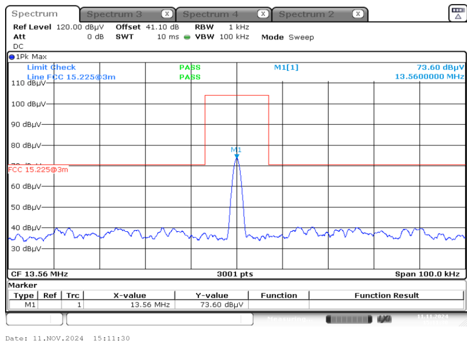
Plot 4: Spectrum mask – span 100 kHz (the limits are recalculated according to the ANSI C63.10-2013 sub clause 6.4)
