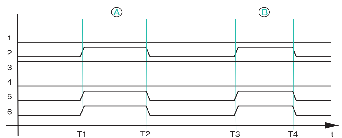
Figure 7.2 Timing sequence of bits in byte 0
