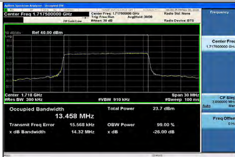
Band4-15MHz-QPSK-20175-75RB#0-29.745
