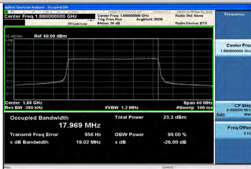
Band2-20MHz-QPSK-19100-100RB#0-17.969
