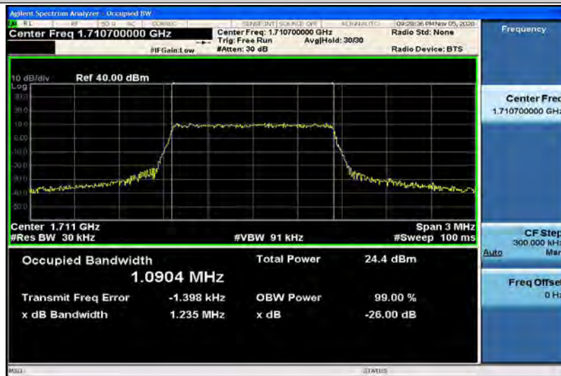
Band4-1.4MHz-16QAM-20175-6RB#0-1.0900
