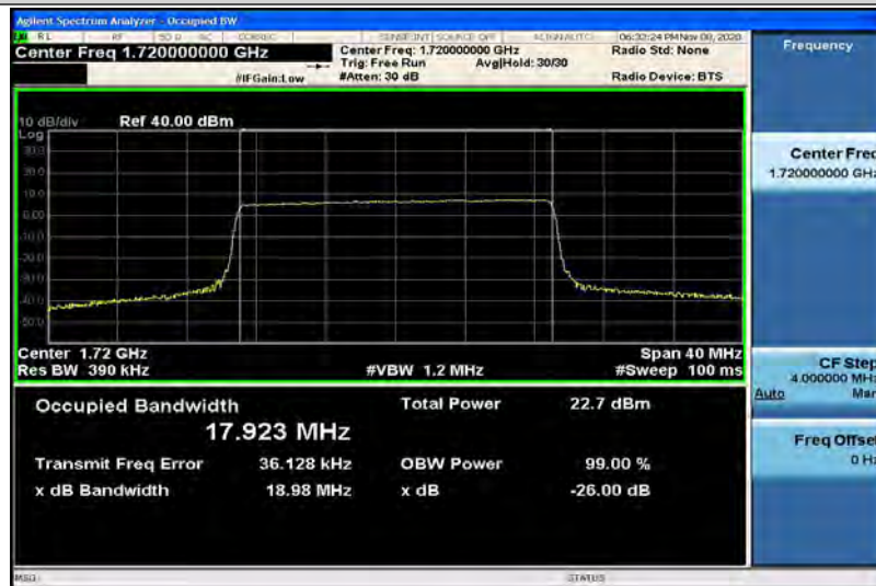
Band4-20MHz-16QAM-20175-100RB#0-39.665
