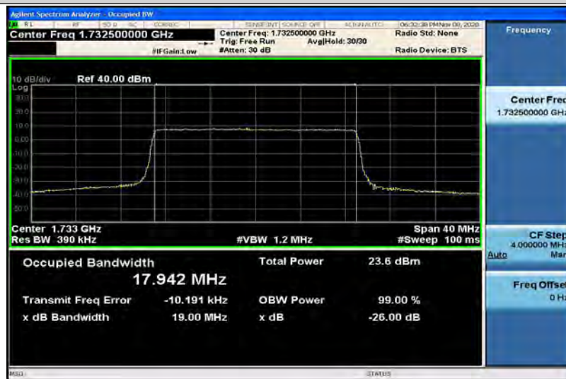
Band4-20MHz-QPSK-20300-100RB#0-17.986
