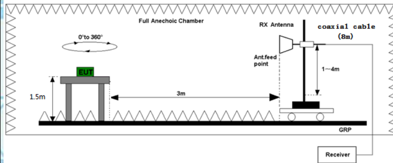
Above 1GHz
