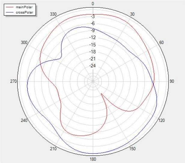
Theta=90 freq=2410MHz
