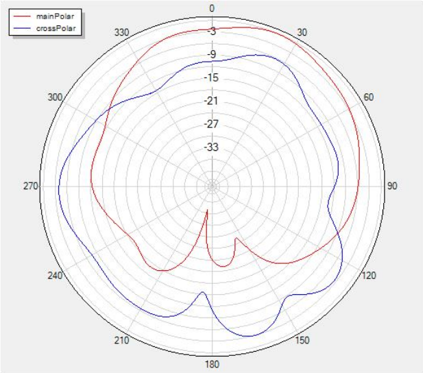
Phi=0 freq=2410MHz
