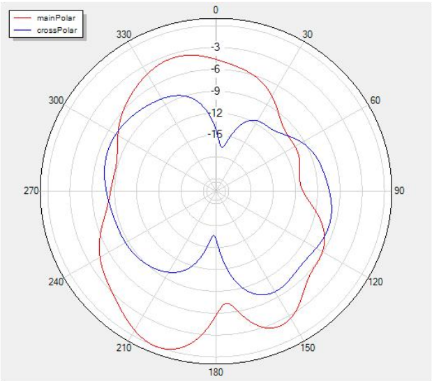
Phi=0 freq=2480MHz
