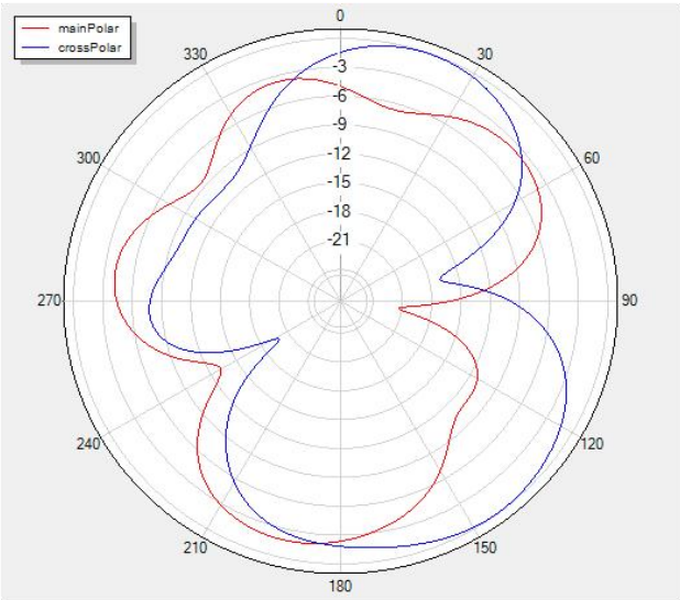
Theta=90 freq=2480MHz
