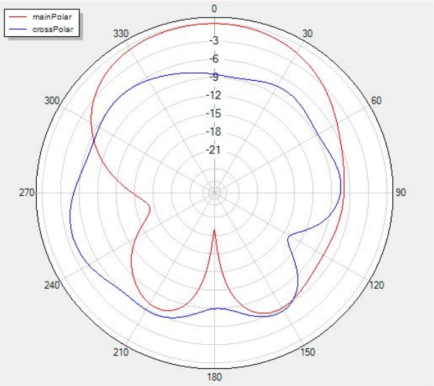
Phi=90 freq=2410MHz
