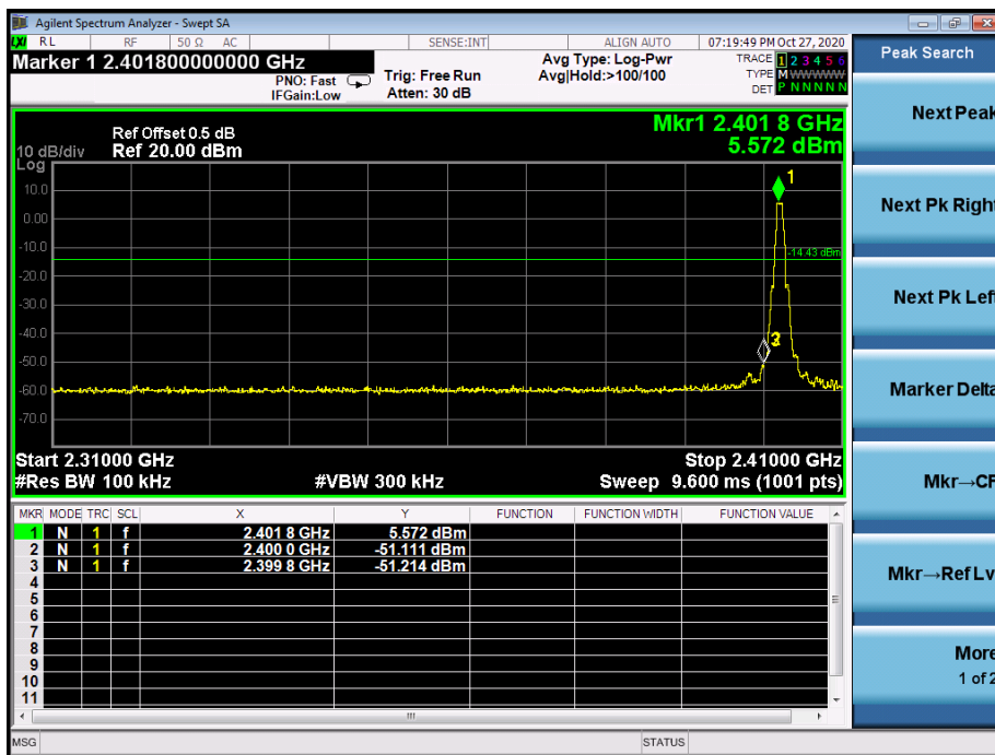
GFSK 1Mbps: Band Edge, Left Side
