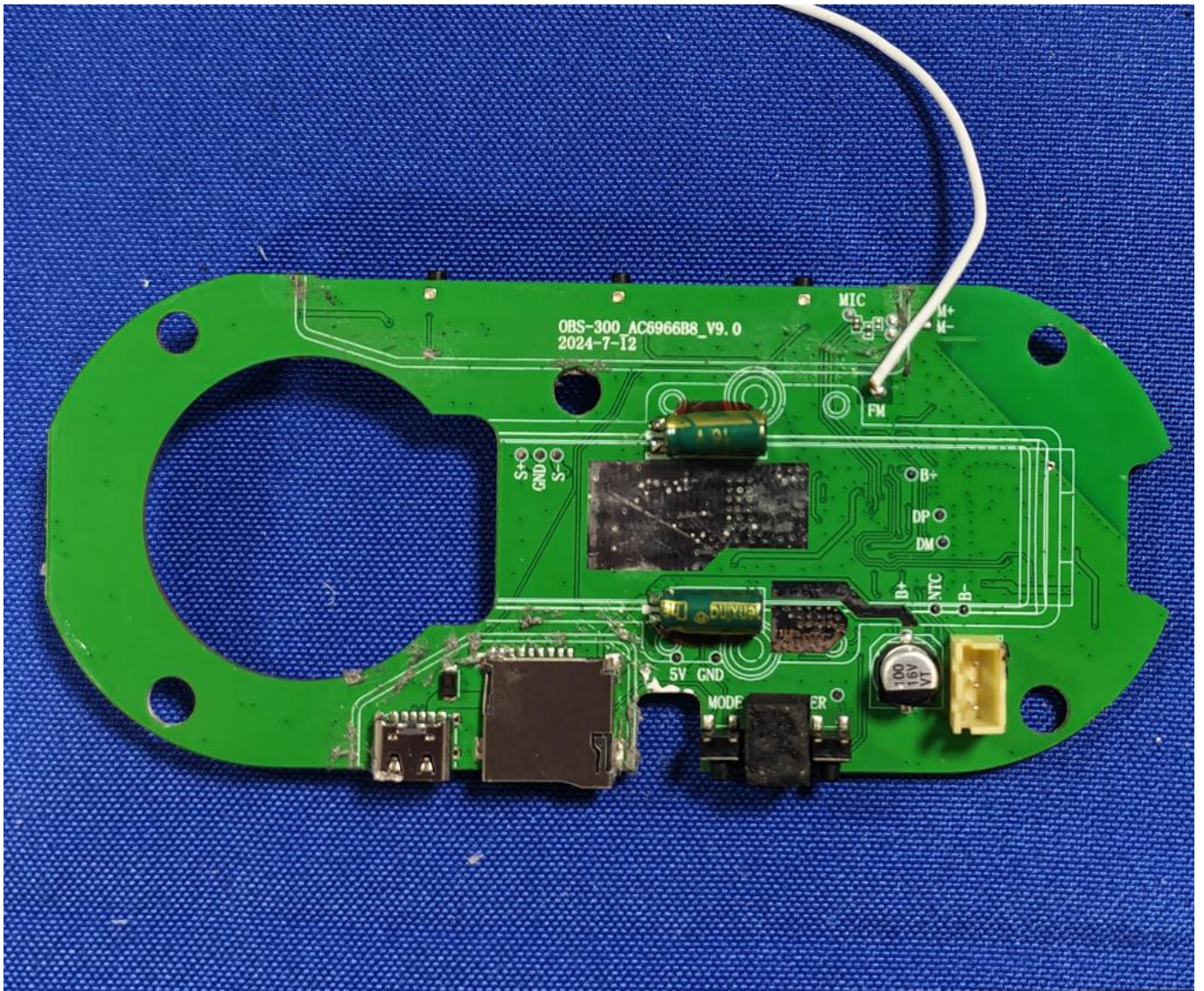
Internal photograph of EUT
